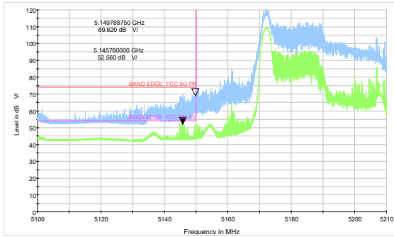
802.11ax HE40-Channel 38 484Tone: Peak + Average
