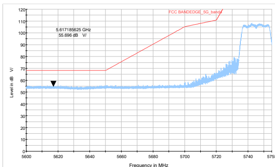
802.11ax HE20-Channel 149 242Tone: Peak
