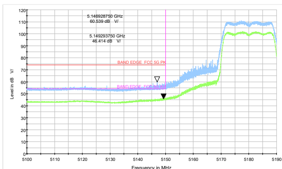
802.11ax HE20-Channel 36 242Tone: Peak + Average
