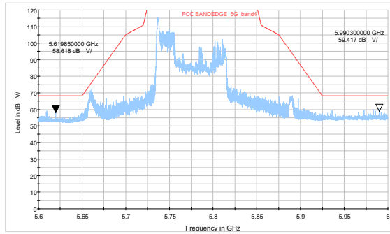
802.11ax HE80-Channel 155 26Tone: Peak
