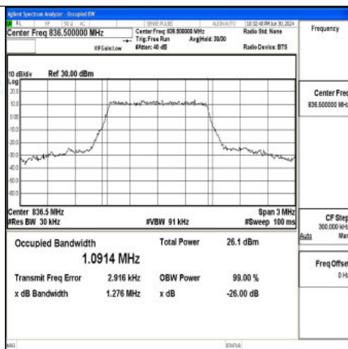
26(824-849)-1.4MHz-16QAM-26915-6RB#0-PASS
