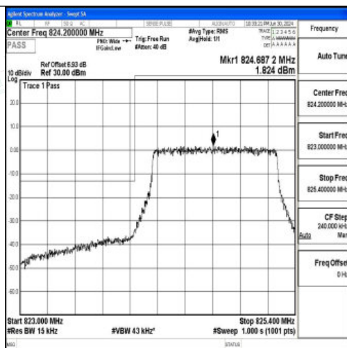
Band26_1.4MHz_16QAM_26797_6RB#0
