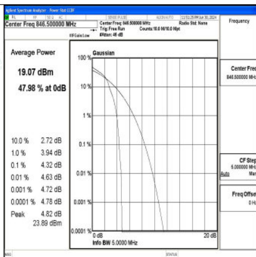
26(824-849)-5MHz-16QAM-27015-1RB#0-PASS
