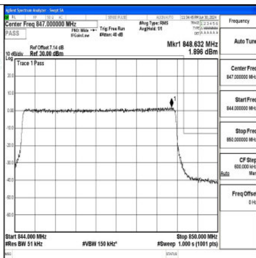
Band26_5MHz_QPSK_27015_25RB#0
