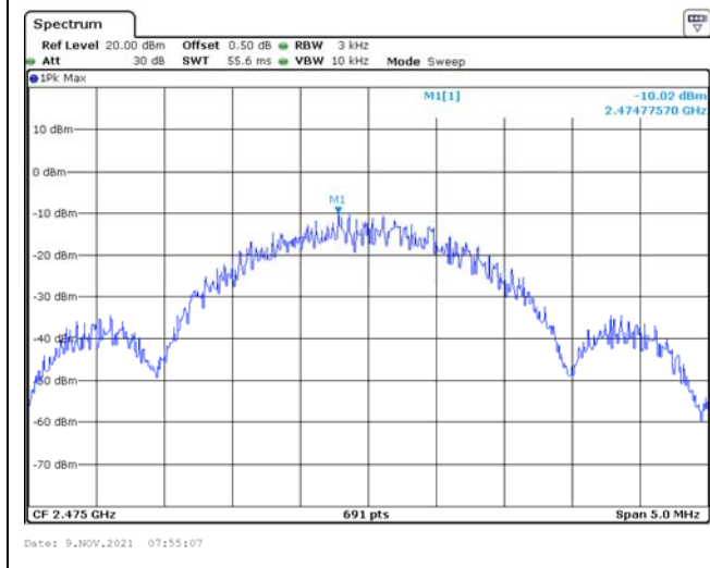
O-QPSK / 2475 MHz
