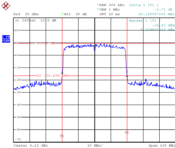
26 dB Bandwidth
