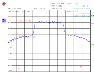
26 dB Bandwidth
