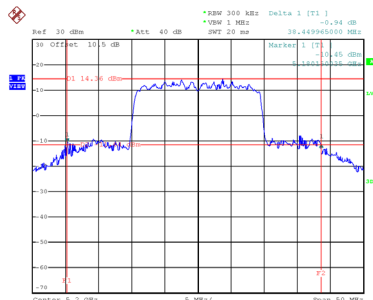
26 dB Bandwidth
