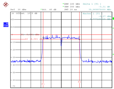
6 dB Bandwidth
