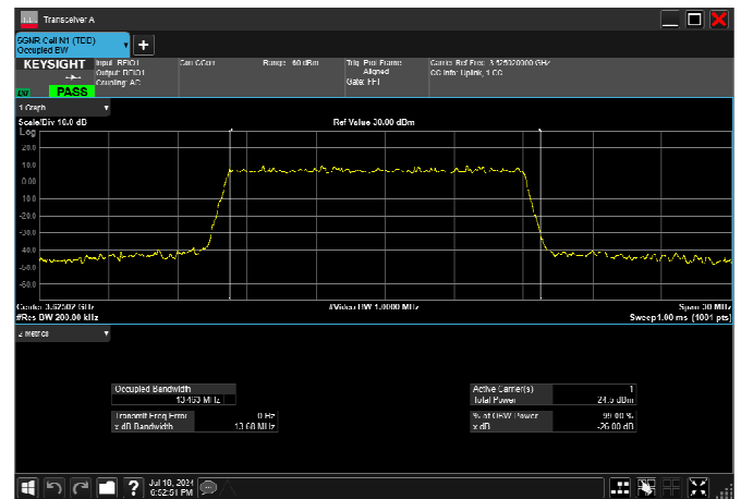
n77_2_15MHz_30kHz_3625MHz_CP-OFDM 16 QAM_RB38@0 13.577MHz
