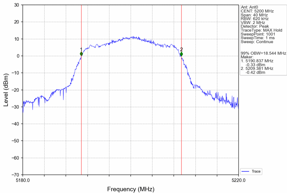
802.11ax(HEW20)_MCH_5200MHz_SU_Ant0_NTNV
