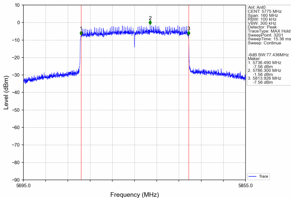
802.11ax(HEW80)_MCH_5775MHz_SU_Ant0_NTNV
