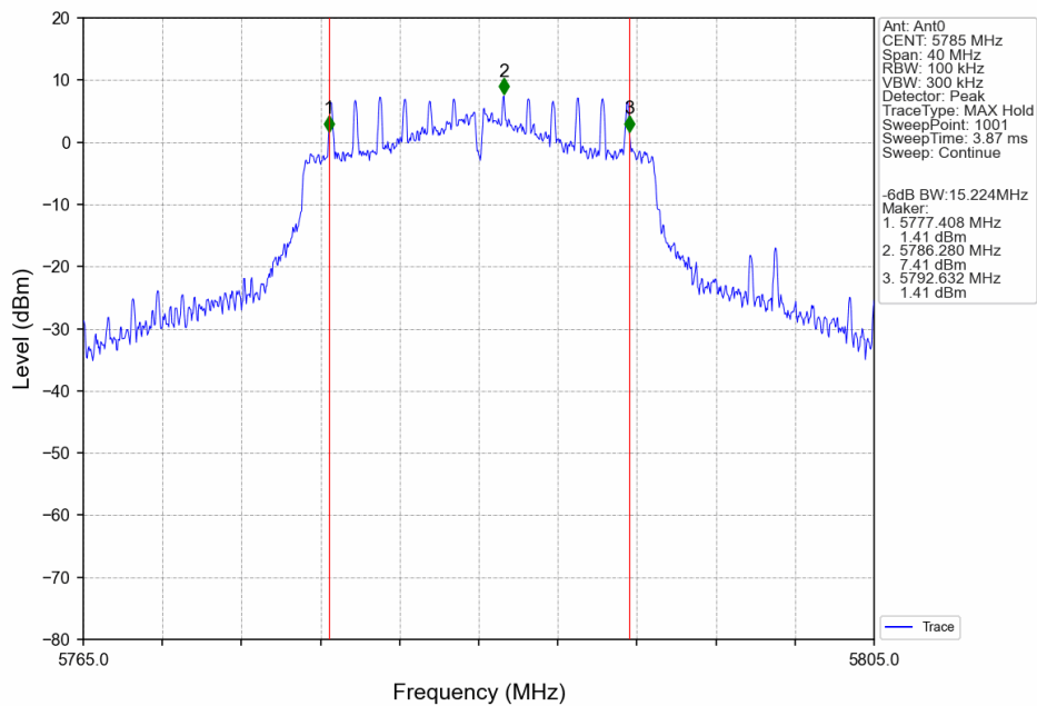
802.11ax(HEW20)_MCH_5785MHz_SU_Ant0_NTNV
