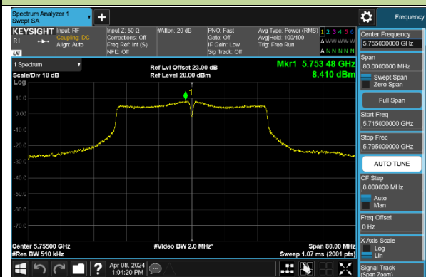
802.11ac-VHT80 Power Spectral Density - Ant 1
