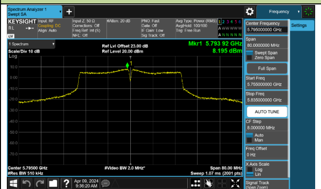
802.11ac-VHT80 Power Spectral Density - Ant 1
