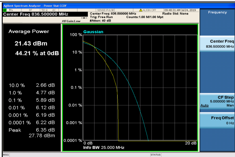
Band5-5MHz-16QAM-20525-1RB#0
