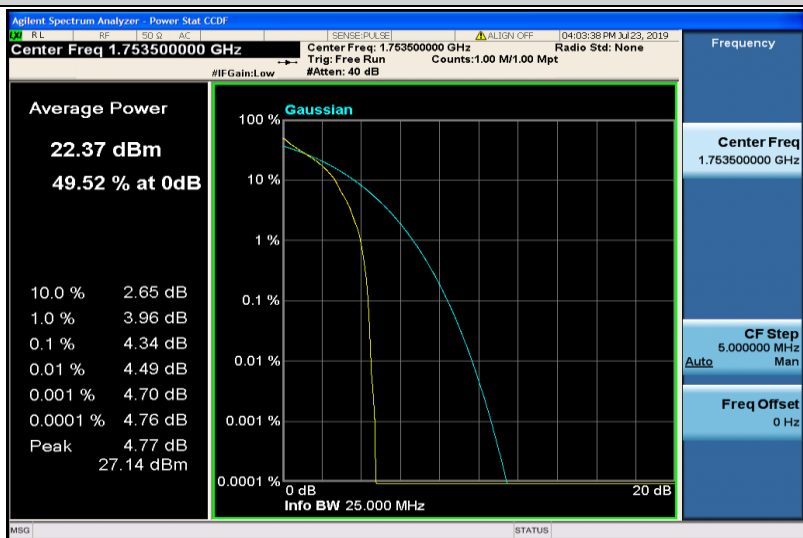
Band4-3MHz-QPSK-20385-1RB#0
