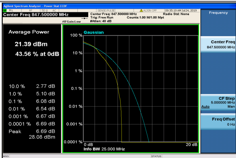
Band5-3MHz-16QAM-20635-1RB#0
