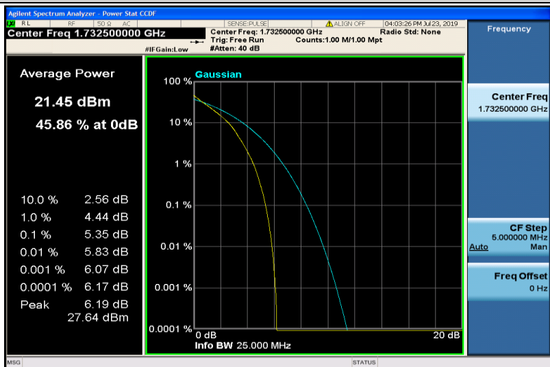
Band4-3MHz-QPSK-20175-15RB#0
