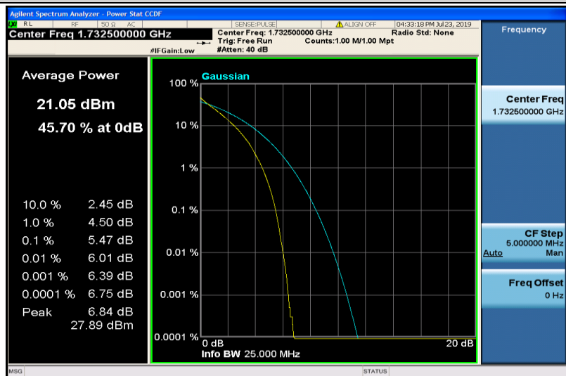
Band4-10MHz-QPSK-20175-50RB#0
