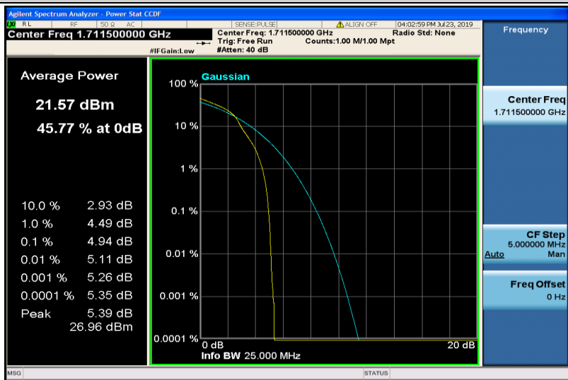
Band4-3MHz-16QAM-19965-1RB#0
