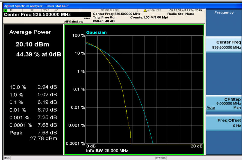
Band5-1.4MHz-16QAM-20525-6RB#0
