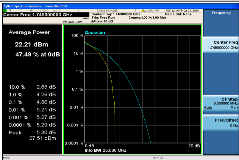
Band4-20MHz-QPSK-20300-1RB#0
