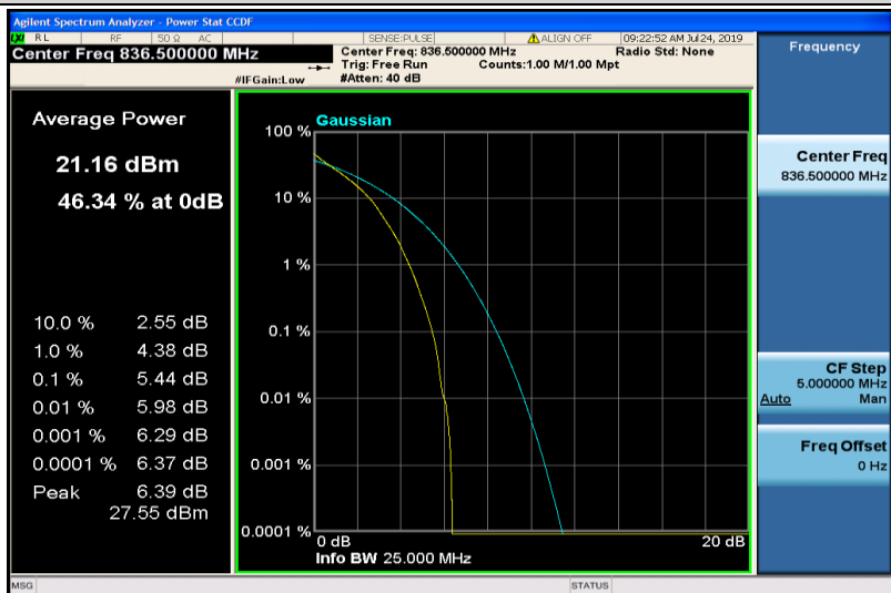
Band5-1.4MHz-QPSK-20525-6RB#0
