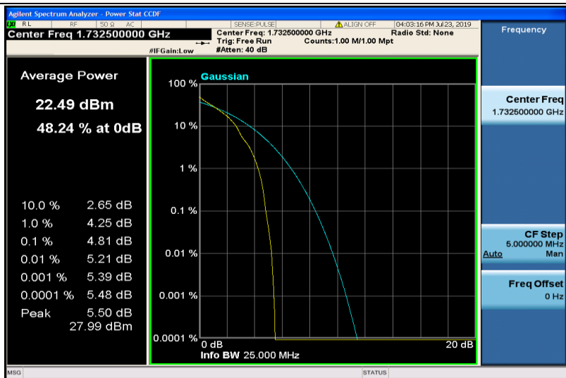
Band4-3MHz-QPSK-20175-1RB#0
