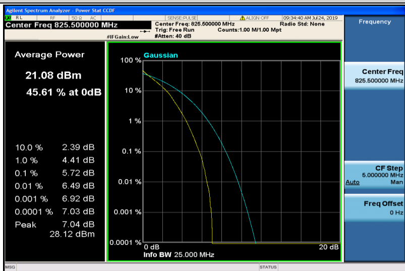
Band5-3MHz-QPSK-20415-15RB#0
