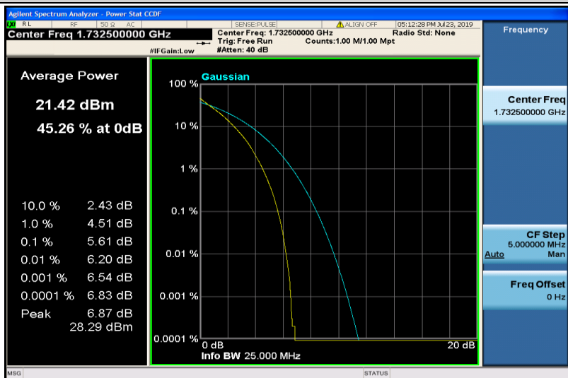
Band4-20MHz-QPSK-20175-100RB#0
