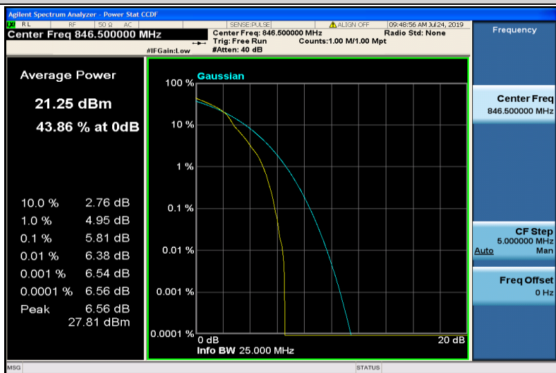
Band5-5MHz-16QAM-20625-1RB#0
