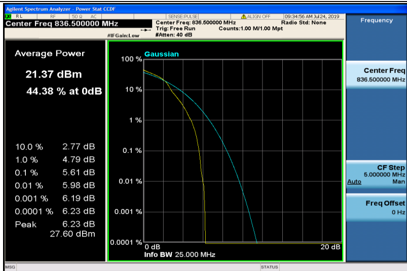
Band5-3MHz-16QAM-20525-1RB#0
