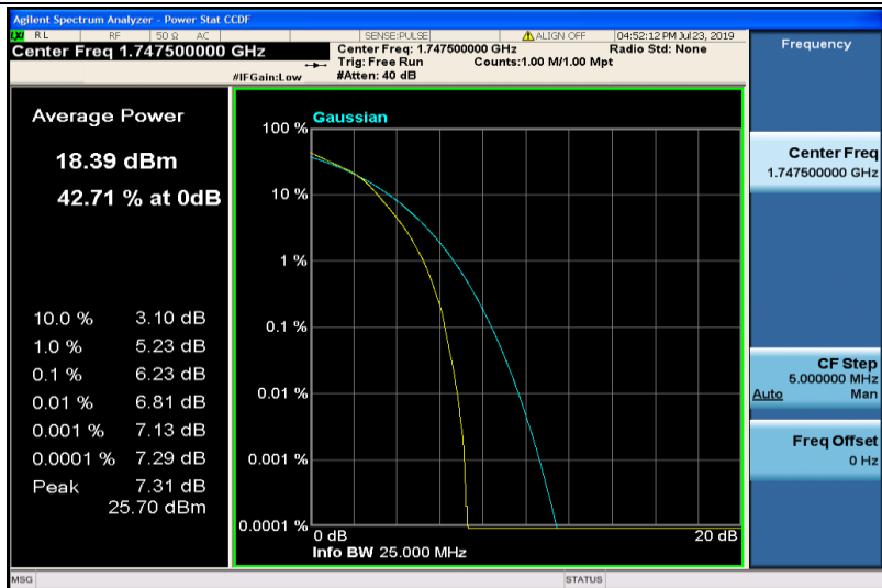
Band4-15MHz-16QAM-20325-75RB#0
