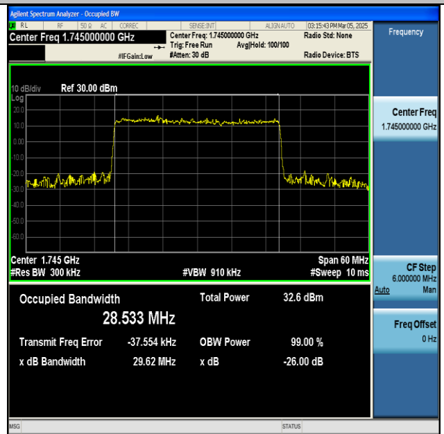
NTNV-n66-PC3-15-30-M-DFT-64QAM-Outer_Full-Ant1- PASS
