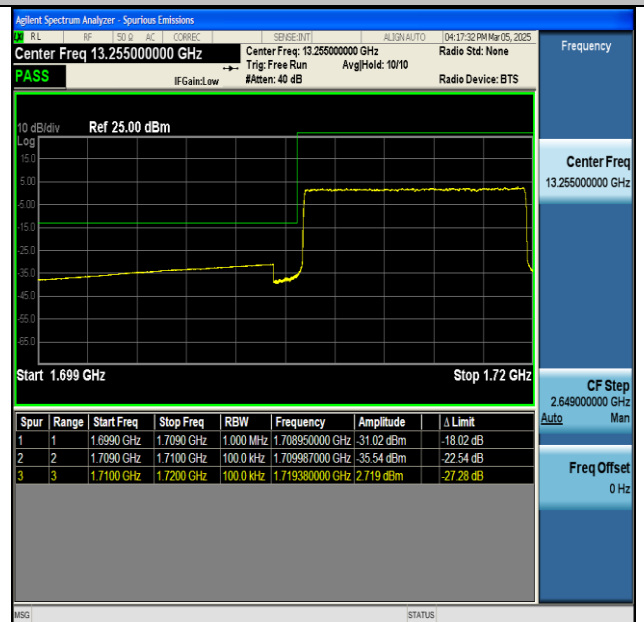
NTNV-n66-PC3-15-10-L-CP-QPSK-Outer_Full-PASS
