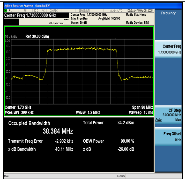
NTNV-n66-PC3-15-40-L-DFT-BPSK-Outer_Full-Ant1- PASS
