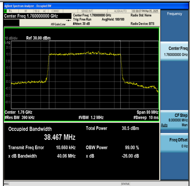
NTNV-n66-PC3-15-40-H-DFT-256QAM-Outer_Full-Ant1-1 PASS
