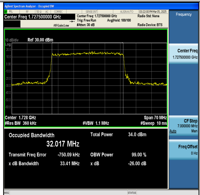
NTNV-n66-PC3-15-35-L-DFT-QPSK-Outer_Full-Ant1- PASS
