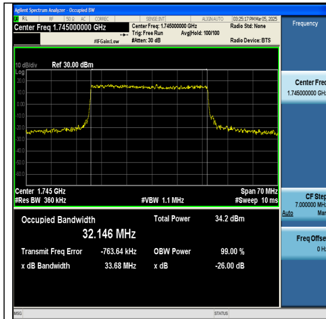
NTNV-n66-PC3-15-35-M-DFT-QPSK-Outer_Full-Ant1- PASS
