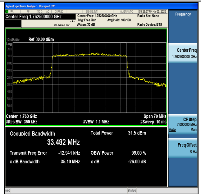
NTNV-n66-PC3-15-35-H-CP-64QAM-Outer_Full-Ant1-PASS
