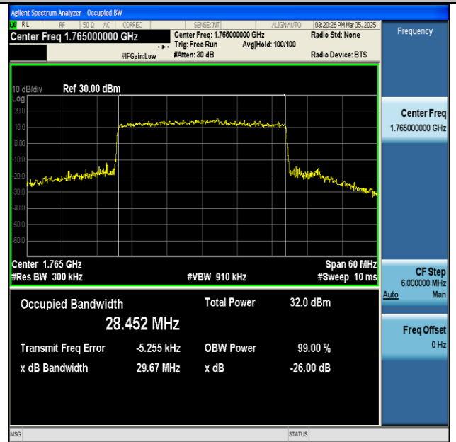
NTNV-n66-PC3-15-30-H-CP-16QAM-Outer_Full-Ant1- PASS
