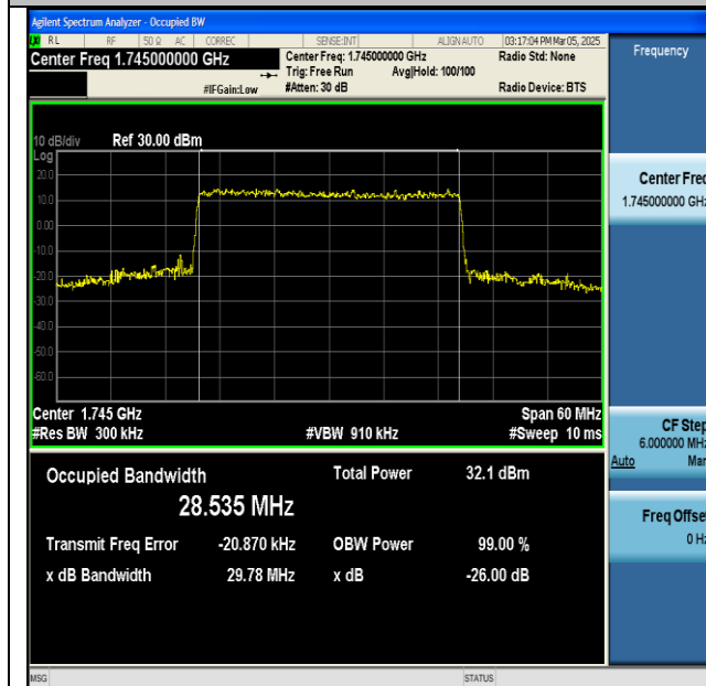
NTNV-n66-PC3-15-30-M-CP-16QAM-Outer_Full-Ant1-PASS
