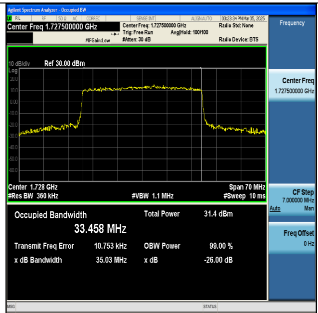
NTNV-n66-PC3-15-35-L-CP-64QAM-Outer_Full-Ant1- PASS
