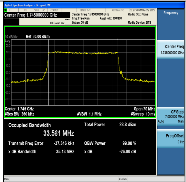
NTNV-n66-PC3-15-35-M-CP-256QAM-Outet_Full-Ant1-PASS
