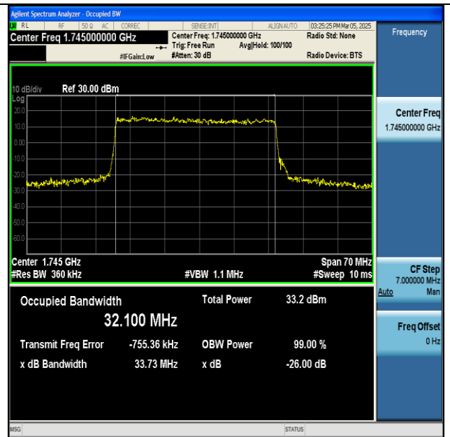
NTNV-n66-PC3-15-35-M-DFT-16QAM-Outer_Full-Ant1- PASS
