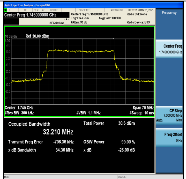
NTNV-n66-PC3-15-35-M-DFT-256QAM-Outer_Full-Ant1- PASS
