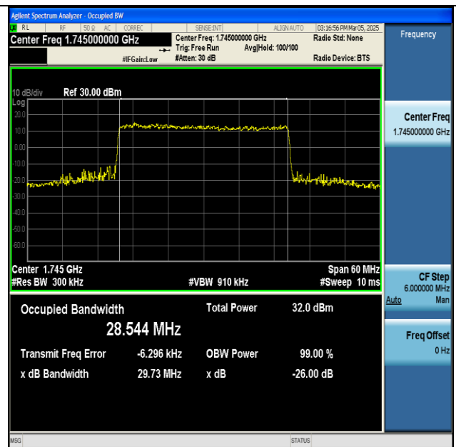
NTNV-n66-PC3-15-30-M-CP-QPSK-Outer_Full-Ant1-PASS
