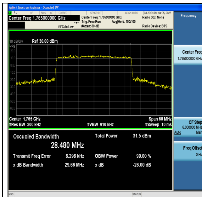
NTNV-n66-PC3-15-30-H-CP-64QAM-Outer_Full-Ant1- PASS
