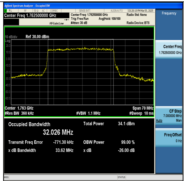
NTNV-n66-PC3-15-35-H-DFT-QPSK-Outer_Full-Ant1- PASS
