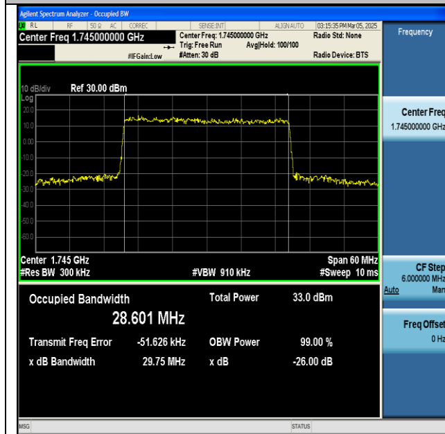
NTNV-n66-PC3-15-30-M-DFT-16QAM-Outer_Full-Ant1- PASS
