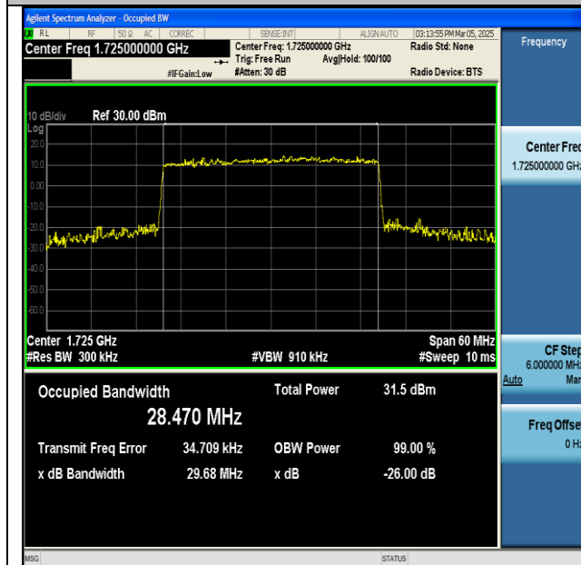
NTNV-n66-PC3-15-30-L-CP-64QAM-Outer_Full-Ant1-PASS
