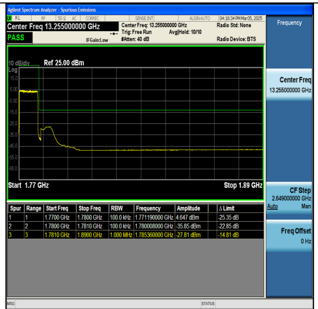
NTNV-n66-PC3-15-10-H-DFT-BPSK-Outer_Full-PASS
