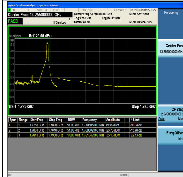
NTNV-n66-PC3-15-5-H-CP-QPSK-Edge_1RB_Right-PASS
