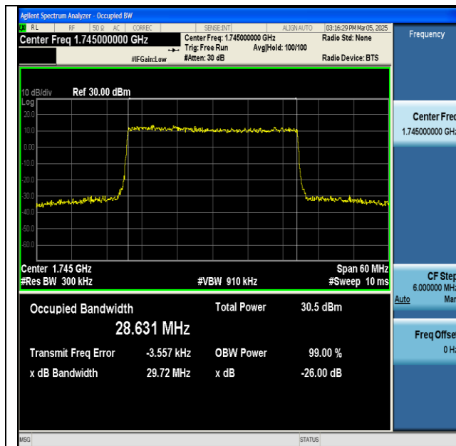
NTNV-n66-PC3-15-30-M-DFT-256QAM-Outer_Full-Ant1-PASS
