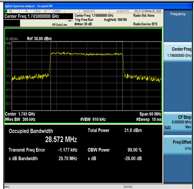
NTNV-n66-PC3-15-30-M-CP-64QAM-Outer_Full-Ant1-PASS
