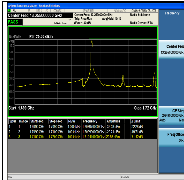
NTNV-n66-PC3-15-10-L-DFT-BPSK-Edge_1RB_Left-PASS
