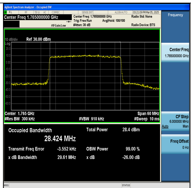
NTNV-n66-PC3-15-30-H-CP-256QAM-Outer_Full-Ant1- PASS
