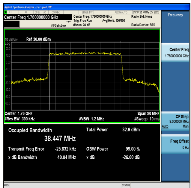
NTNV-n66-PC3-15-40-H-DFT-16QAM-Outer_Full-Ant1-1 PASS
