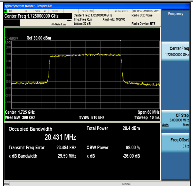
NTNV-n66-PC3-15-30-L-CP-256QAM-Outer_Full-Ant1-PASS
