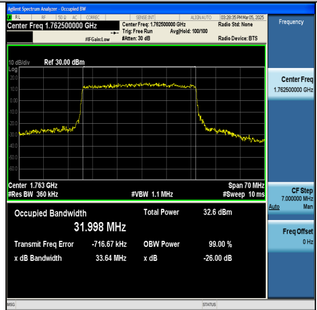
NTNV-n66-PC3-15-35-H-DFT-64QAM-Outer_Full-Ant1- PASS
