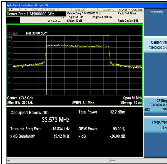
NTNV-n66-PC3-15-35-M-CP-QPSK-Outet_Full-Ant1-PASS
