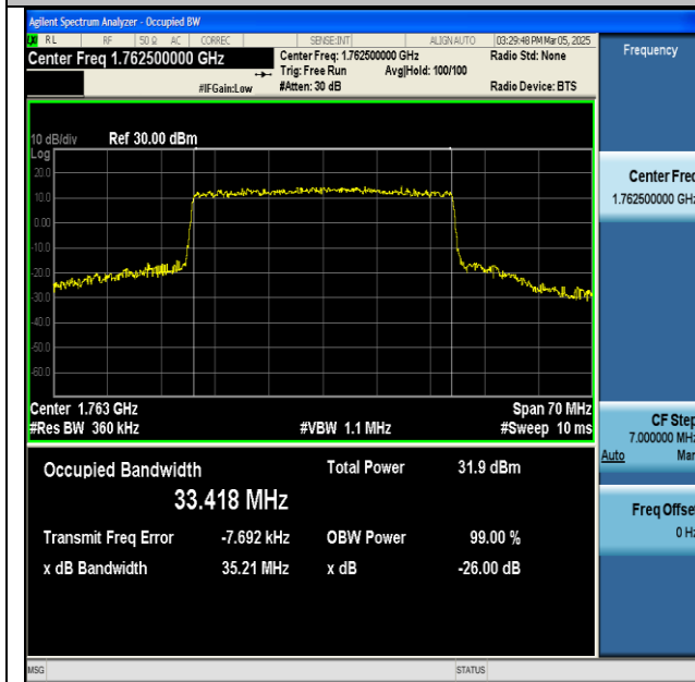
NTNV-n66-PC3-15-35-H-CP-16QAM-Outer_Full-Ant1-PASS
