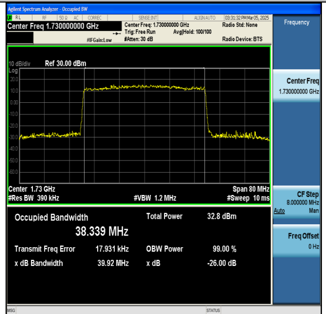
NTNV-n66-PC3-15-40-L-DFT-16QAM-Outer_Full-Ant1- PASS
