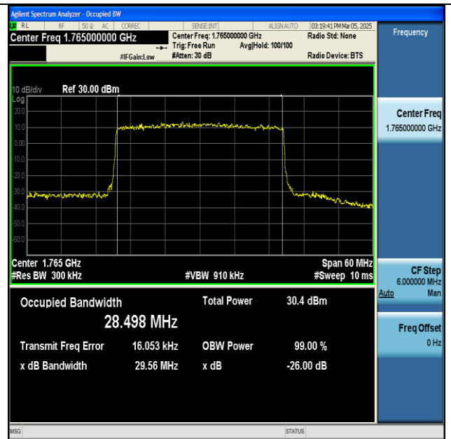
NTNV-n66-PC3-15-30-H-DFT-256QAM-Outer_Full-Ant1- PASS
