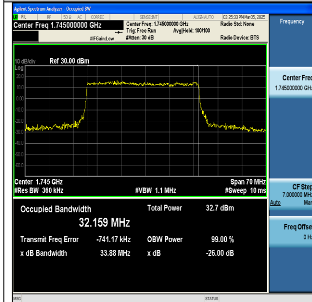
NTNV-n66-PC3-15-35-M-DFT-64QAM-Outer_Full-Ant1- PASS
