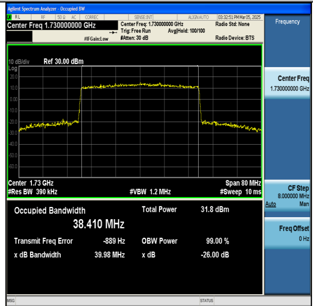
NTNV-n66-PC3-15-40-L-CP-16QAM-Outer_Full-Ant1- PASS
