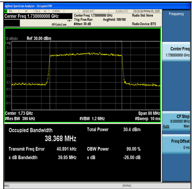
NTNV-n66-PC3-15-40-L-DFT-256QAM-Outer_Full-Ant1- PASS
