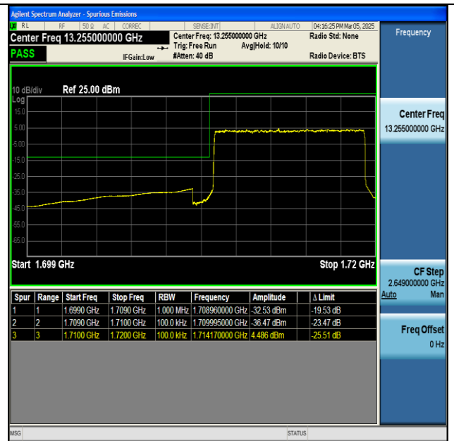
NTNV-n66-PC3-15-10-L-DFT-BPSK-Outer_Full-PASS
