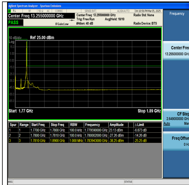
NTNV-n66-PC3-15-10-H-DFT-BPSK-Edge_1RB_Right-PASS
