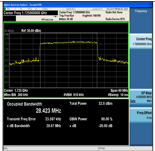
NTNV-n66-PC3-15-30-L-CP-16QAM-Outer_Full-Ant1-PASS
