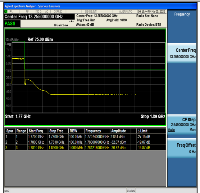
NTNV-n66-PC3-15-10-H-CP-QPSK-Outer_Full-PASS
