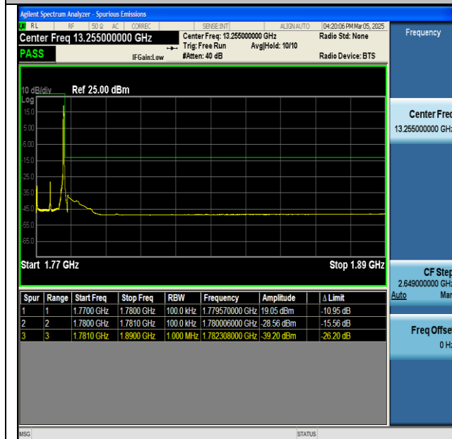
NTNV-n66-PC3-15-10-H-CP-QPSK-Edge_1RB_Right-PASS
