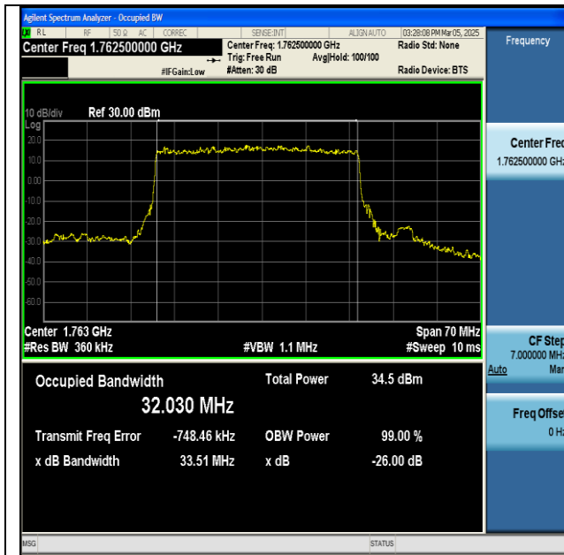
NTNV-n66-PC3-15-35-H-DFT-BPSK-Outer_Full-Ant1- PASS
