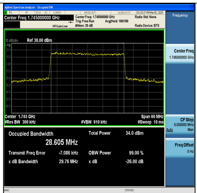
NTNV-n66-PC3-15-30-M-DFT-QPSK-Outer_Full-Ant1- PASS
