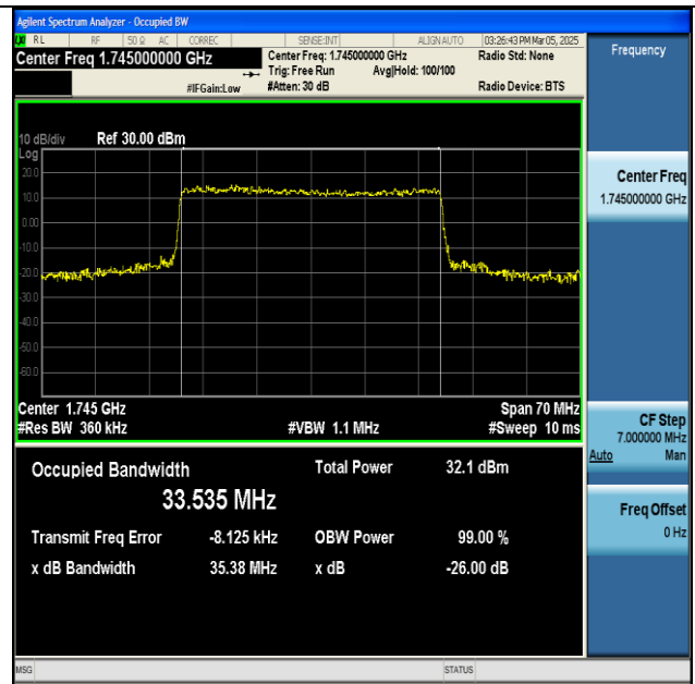
NTNV-n66-PC3-15-35-M-CP-16QAM-Outet_Full-Ant1-PASS
