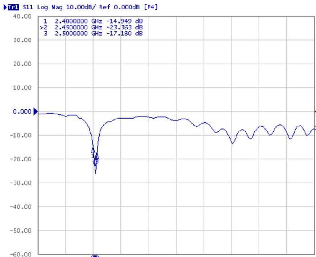
Figure 2 Return Loss
