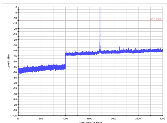
LTE Band 4 1.4MHz CH-Middle 30MHz~3GHz
