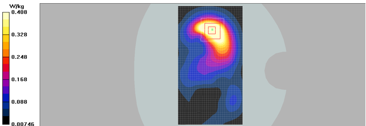
Fig.4 GSM 1900 MHz CH810
