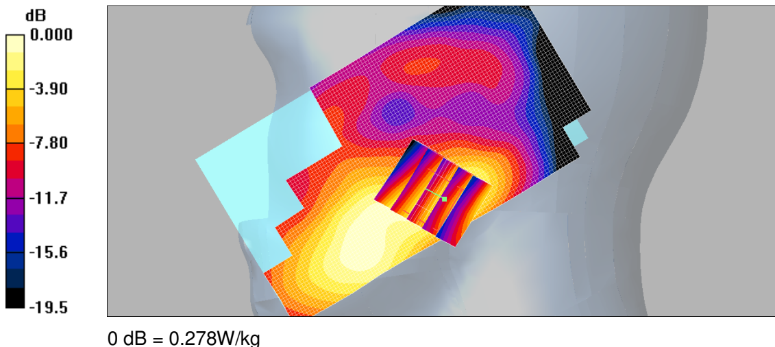
Fig.9 LTE Band 2 CH18900
