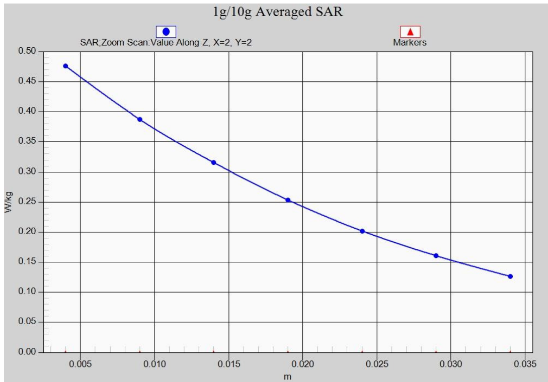
Fig.17-1 Z-Scan at power reference point (Band 12 CH23095)
