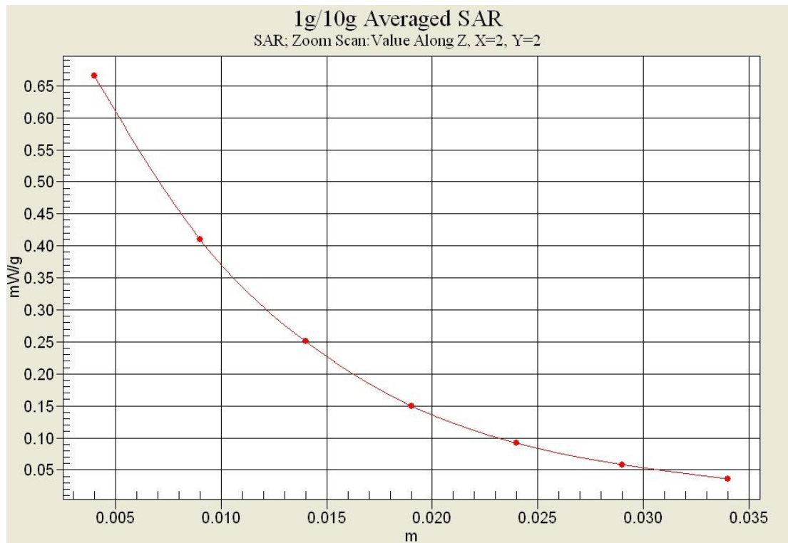
Fig.10-1 Z-Scan at power reference point (Band 2 CH18900)
