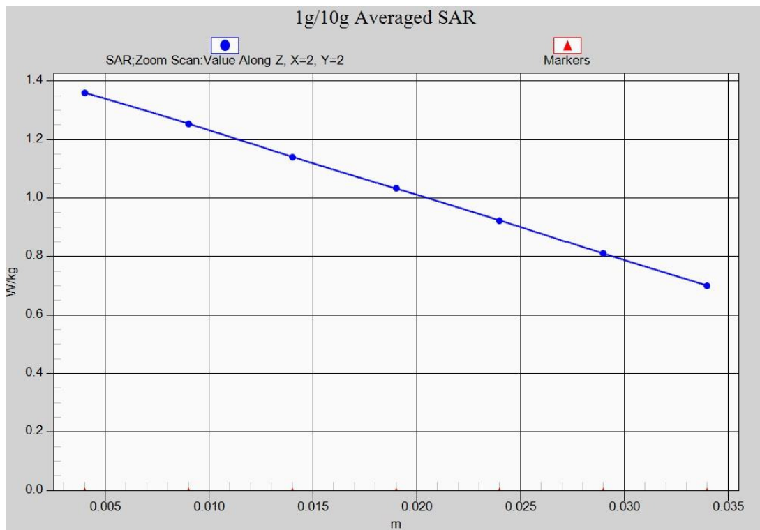
Fig.16-1 Z-Scan at power reference point (Band 7 CH21350)
