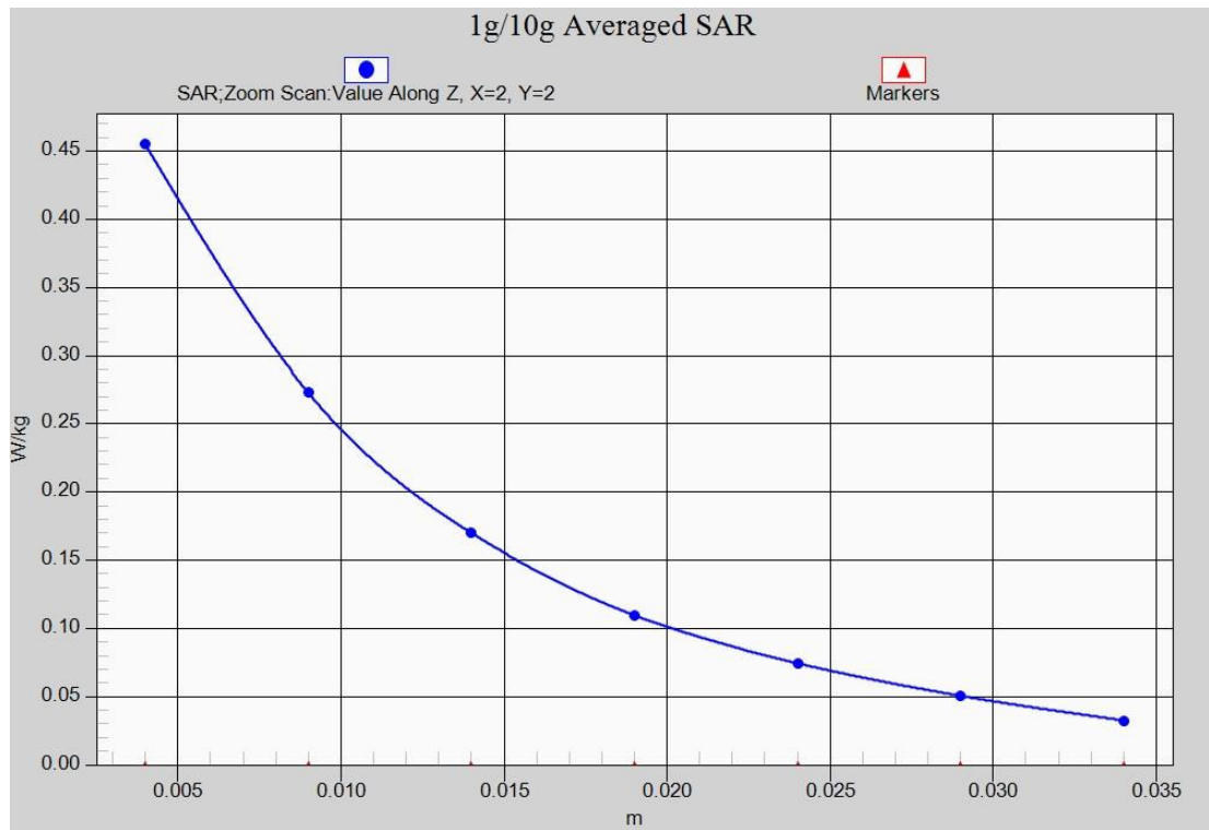
Fig.2-1 Z-Scan at power reference point (GSM 850 MHz CH128)
