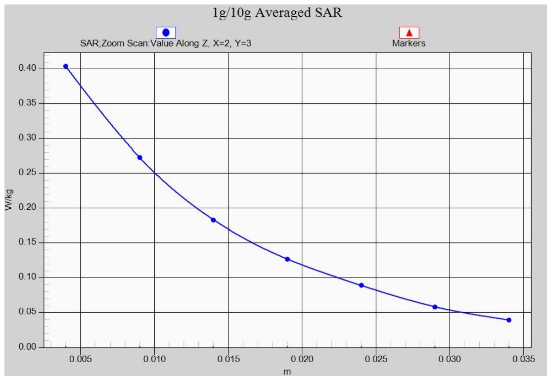
Fig.4-1 Z-Scan at power reference point (GSM 1900 MHz CH810)
