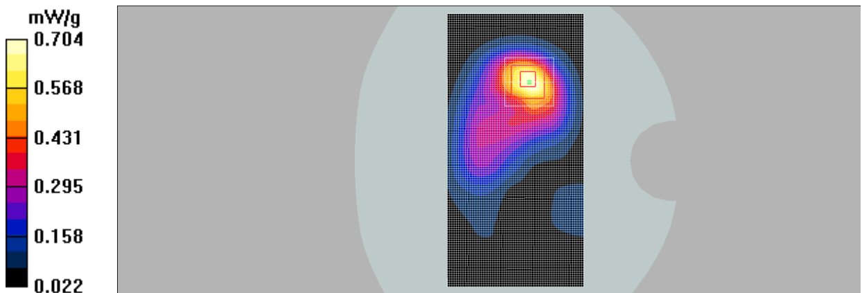
Fig.12 LTE Band 4 CH20175
