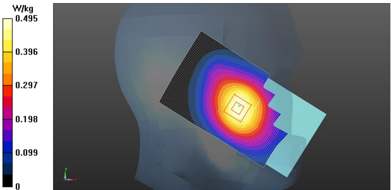
Fig.17 LTE Band 12 CH23095
