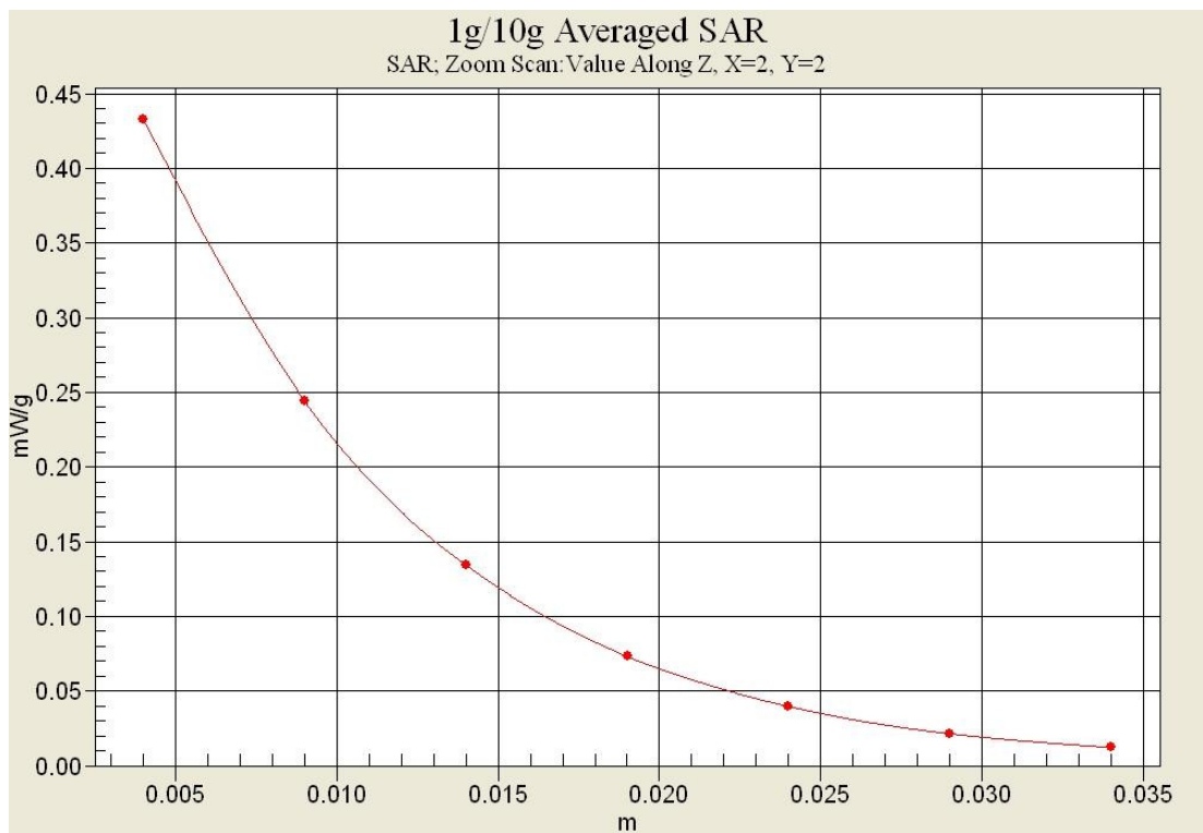
Fig.15-1 Z-Scan at power reference point (Band 7 CH20850)
