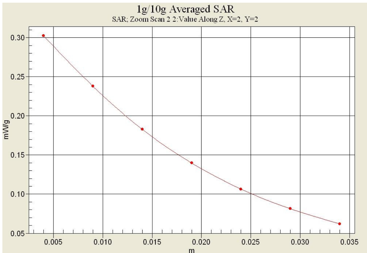
Fig.6-1 Z-Scan at power reference point (WCDMA850 CH4132)
