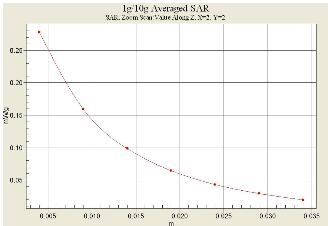
Fig.9-1 Z-Scan at power reference point (Band 2 CH18900)
