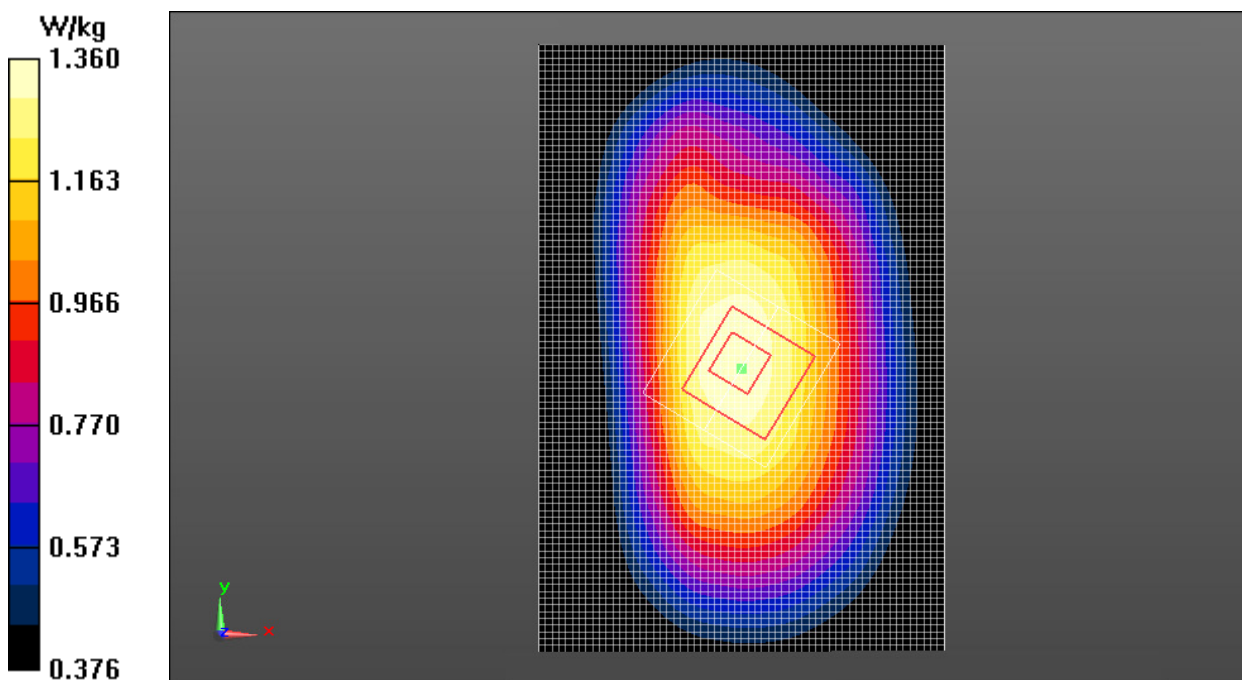
Fig.16 LTE Band 7 CH21350
