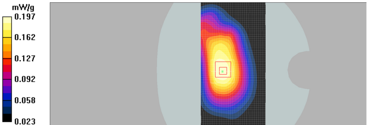
Fig.14 LTE Band 5 CH20600
