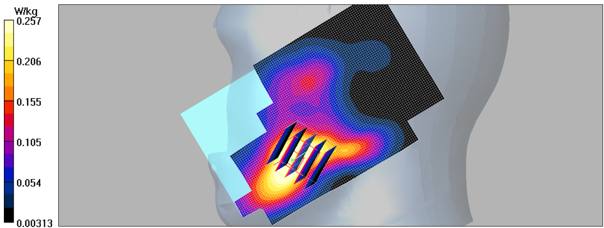
Fig.11 LTE Band4 CH20175
