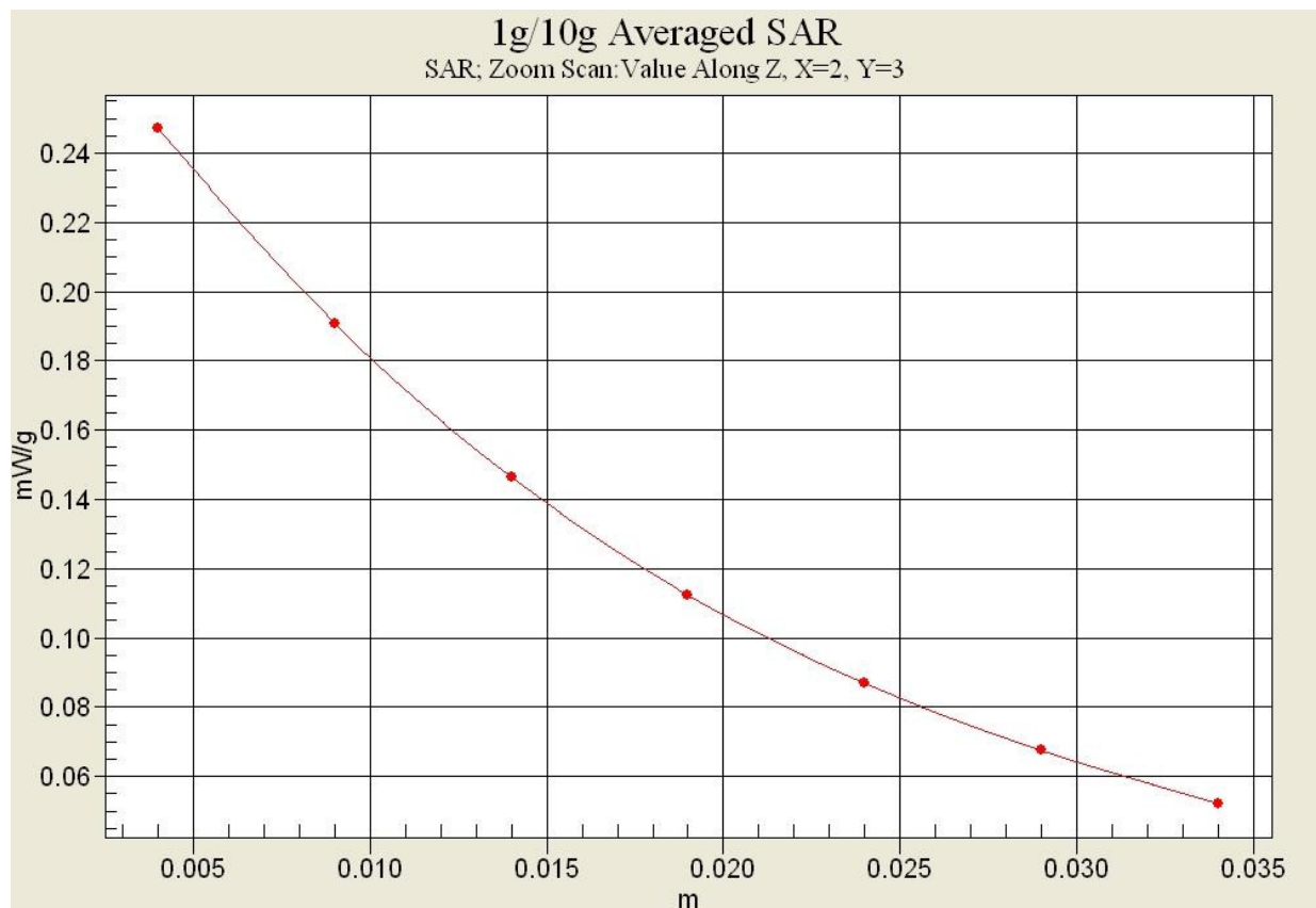
Fig.13-1 Z-Scan at power reference point (Band 5 CH20600)
