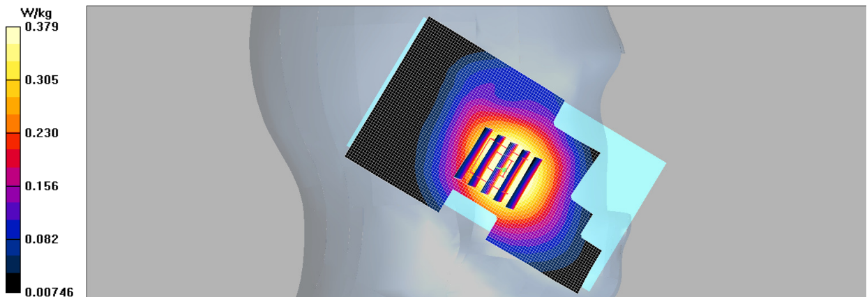
Fig.1 GSM 850MHz CH128
