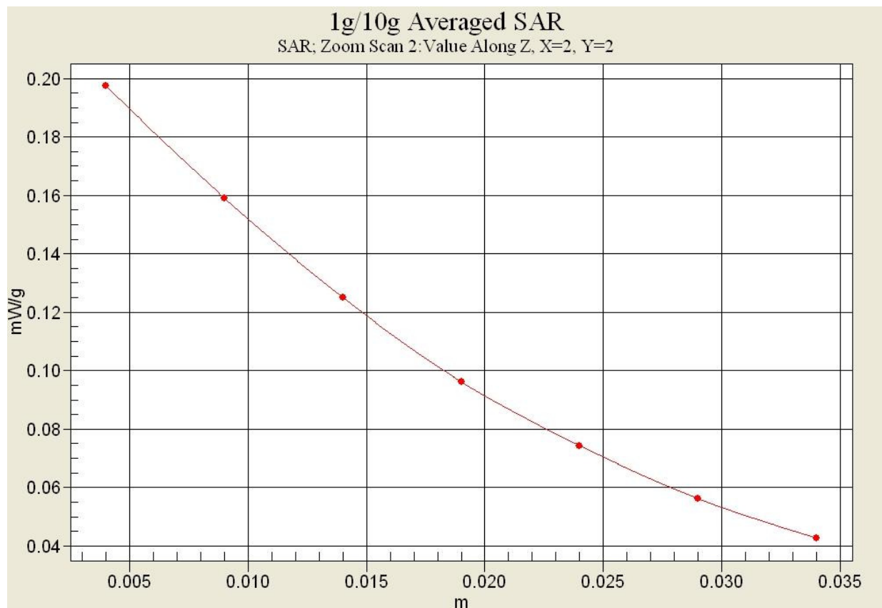
Fig.14-1 Z-Scan at power reference point (Band 5 CH20600)
