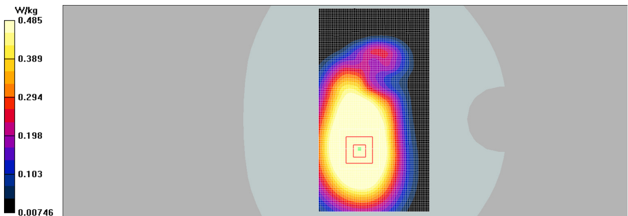
Fig.2 GSM 850 MHz CH128
