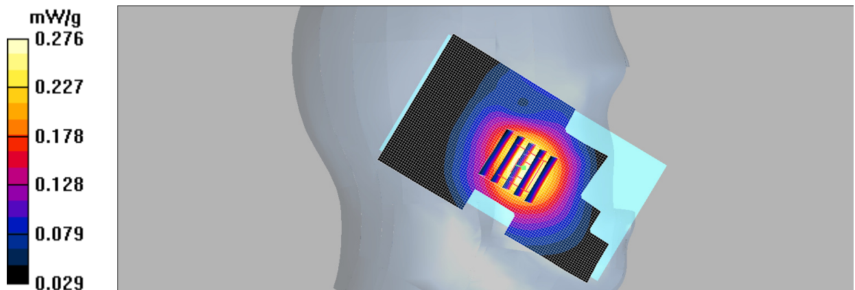
Fig.5 WCDMA 850 CH4233
