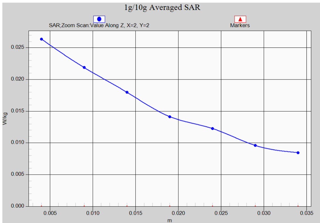
Fig.11-1 Z-Scan at power reference point (Band 4 CH20175)
