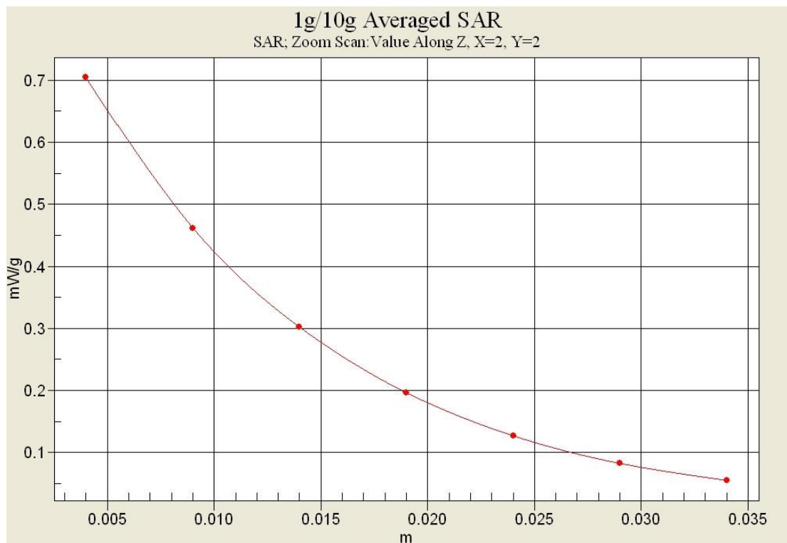
Fig.12-1 Z-Scan at power reference point (Band 4 CH20175)
