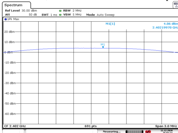
Figure 3: Maximum peak Conducted Output Power
