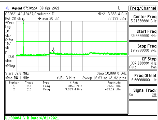
5G NR n12 5MHz BPSK Middle Channel RB1-1
