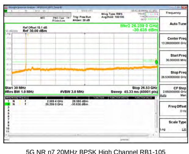
5G NR n7 20MHz BPSK High Channel RB1-105
