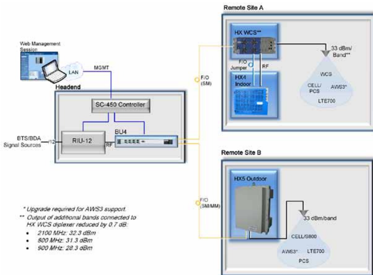
Example of SISO Architecture with HX4 Indoor, HX WCS, and HX5 Outdoor Figure 1-2
