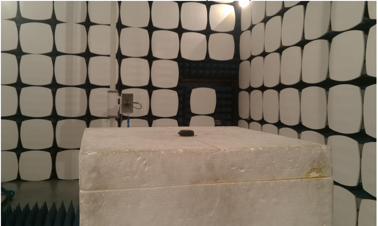
Radiated Emission(above 1G)
