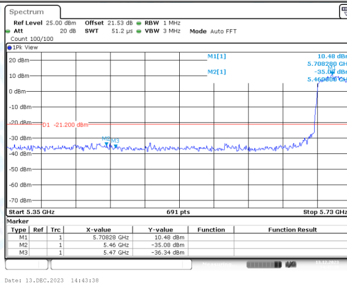
11N40SISO_Ant1_High_5710_Peak
