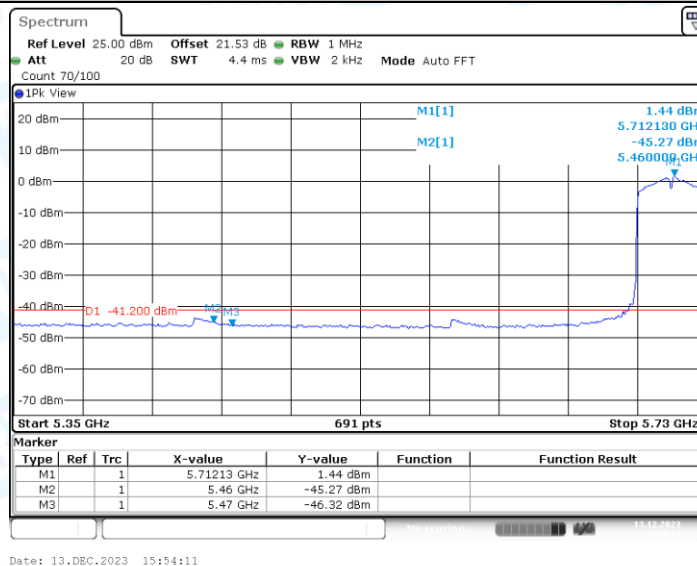
11AC40SISO_Ant1_Low_5710_Peak
