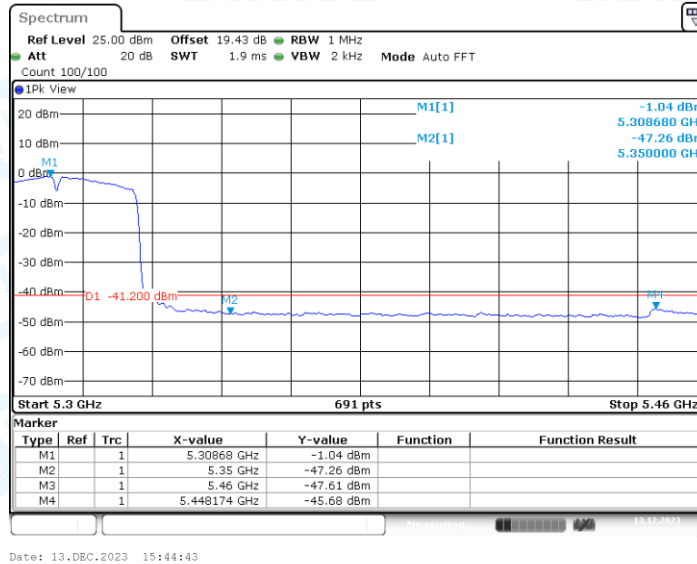
11AC40SISO_Ant1_High_5310_Peak
