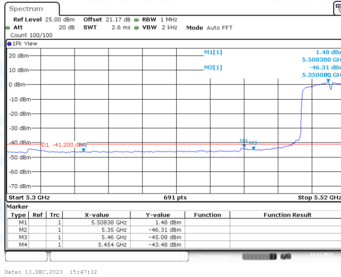
11AC40SISO_Ant1_Low_5510_Peak
