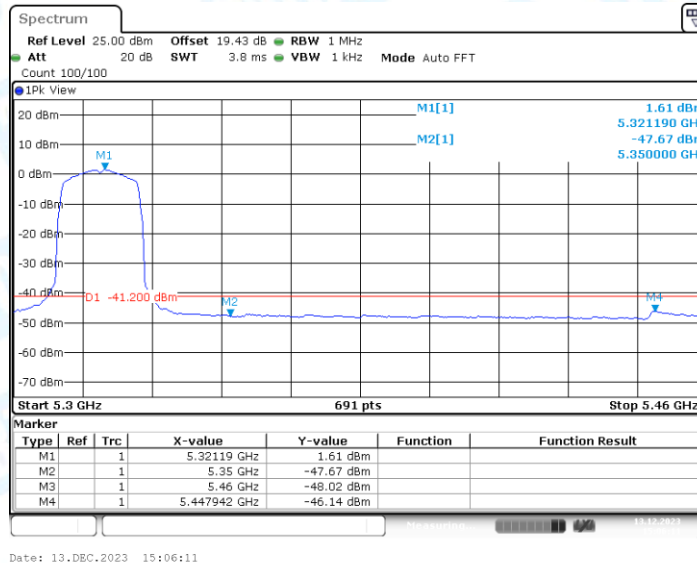
11AC20SISO_Ant1_High_5320_Peak
