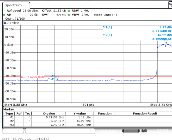
11N40SISO_Ant1_Low_5710_Peak
