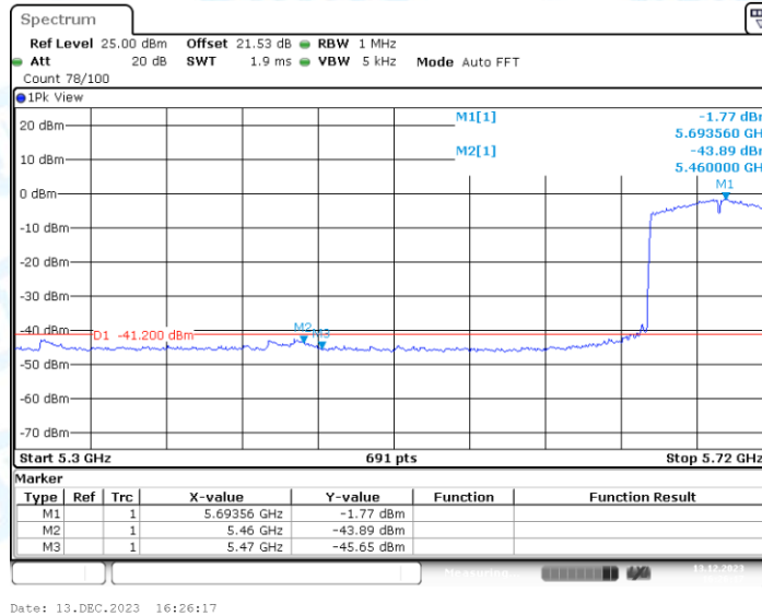
11AC80SISO_Ant1_Low_5690_Peak
