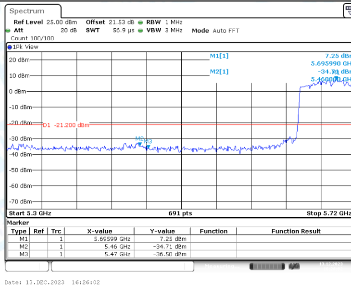
11AC80SISO_Ant1_High_5690_Peak
