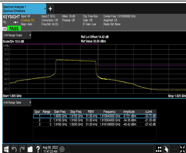
Band25-5MHz-16QAM-26665-25RB#0
