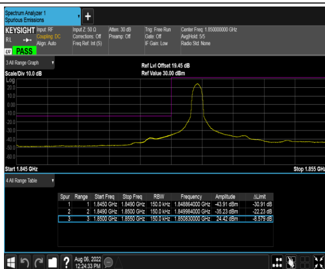
Band25-15MHz-16QAM-26115-75RB#0
