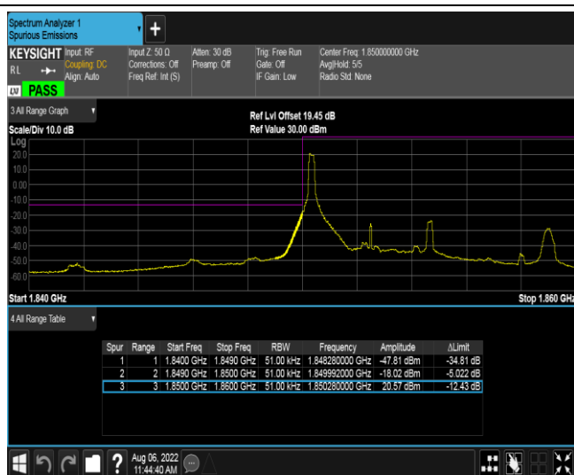
Band25-5MHz-QPSK-26065-25RB#0
