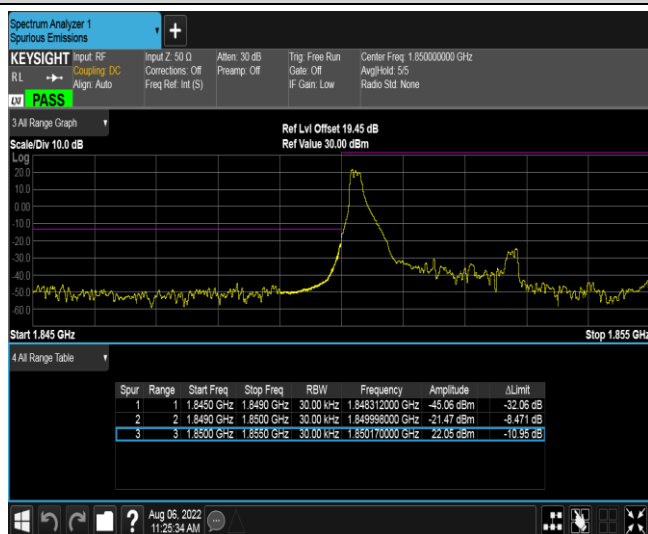
Band25-3MHz-QPSK-26055-1RB#0
