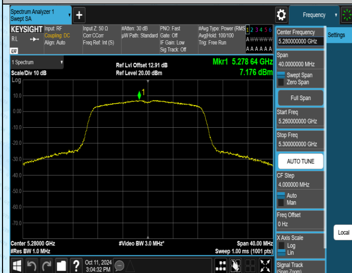
11N20SISO-Ant1-5280-PASS
