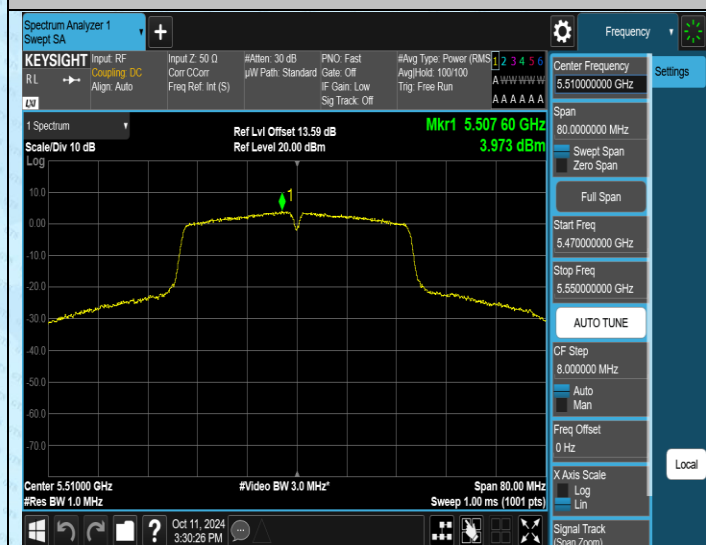
11N40SISO-Ant1-5510-PASS
