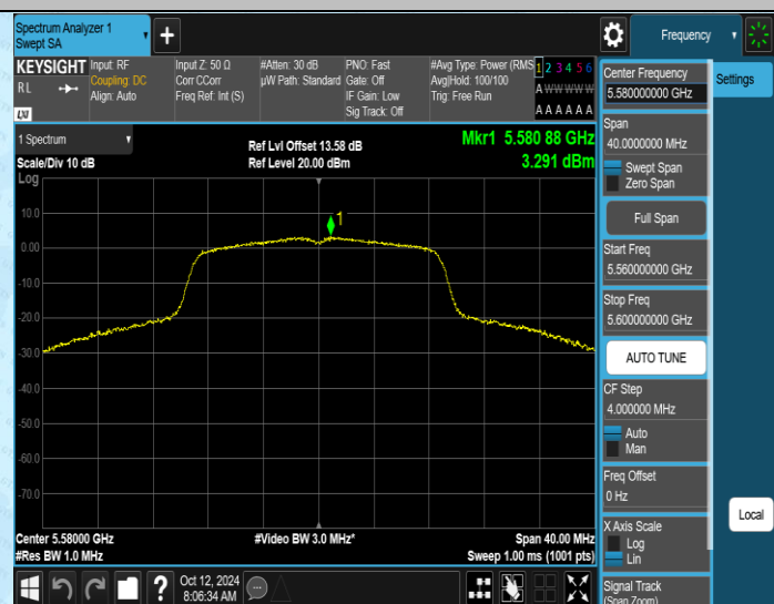
11N20SISO-Ant2-5580-PASS
