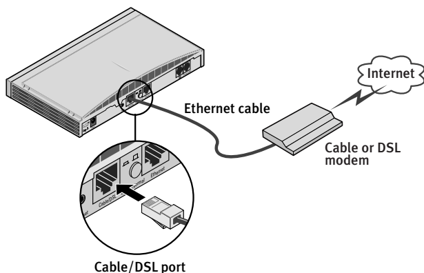
Figure 7 Cable or DSL Modem Connected to the Gateway
