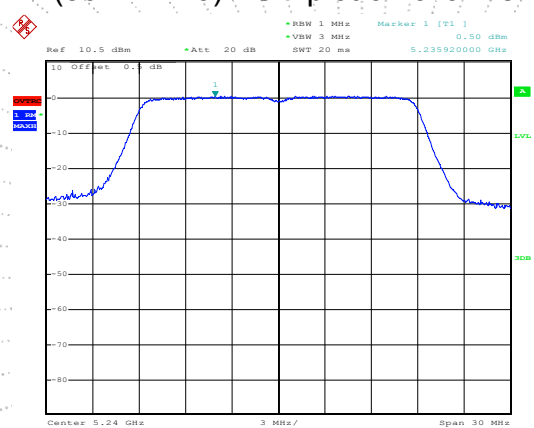
(802.11n20) PSD plot on channel 48
