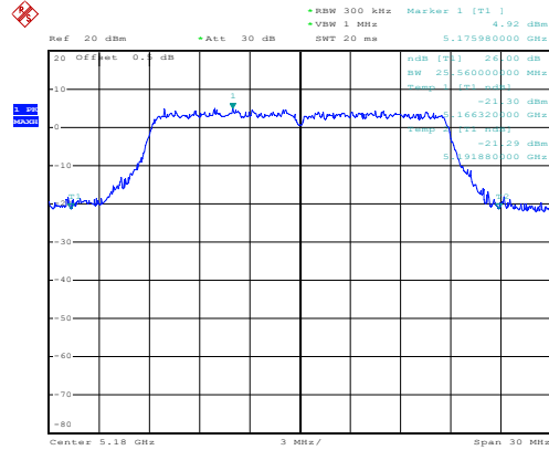
(802.11a) 26dB Bandwidth plot on channel 36
