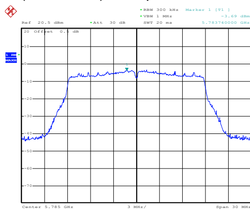
(802.11n20) PSD plot on channel 157
