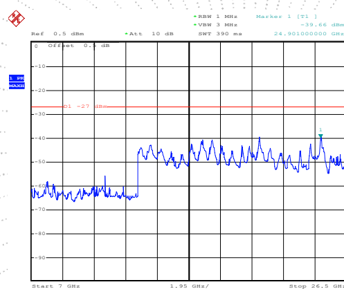
802.11a on channel 157
