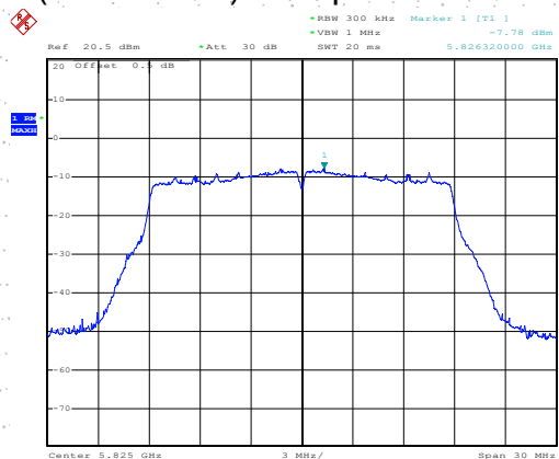
(802.11ac20) PSD plot on channel 165
