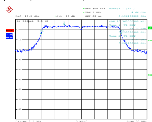
(802.11a) 99%Bandwidth plot on channel 40
