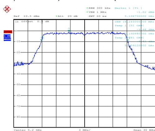
(802.11 AC20) 99%Bandwidth plot on channel 40
