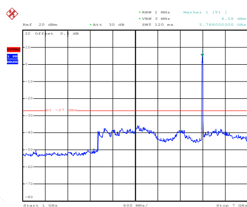
802.11ac20 on channel 157
