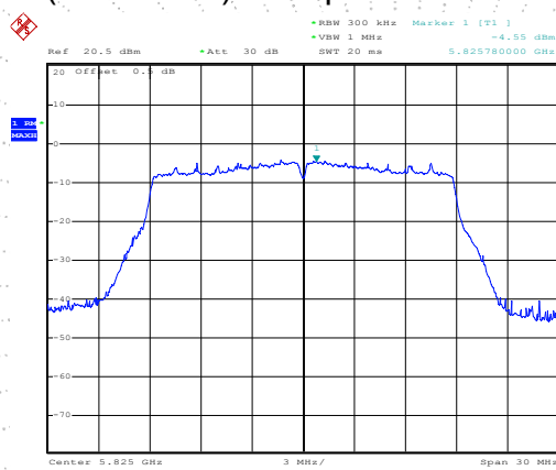
(802.11n20) PSD plot on channel 165
