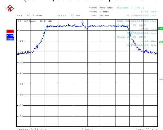
(802.11a) 99%Bandwidth plot on channel 48
