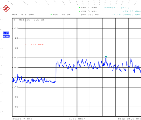
802.11n40 on channel 46
