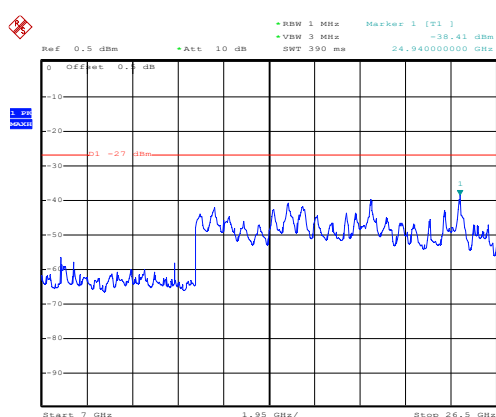
802.11 ac40 on channel 46
