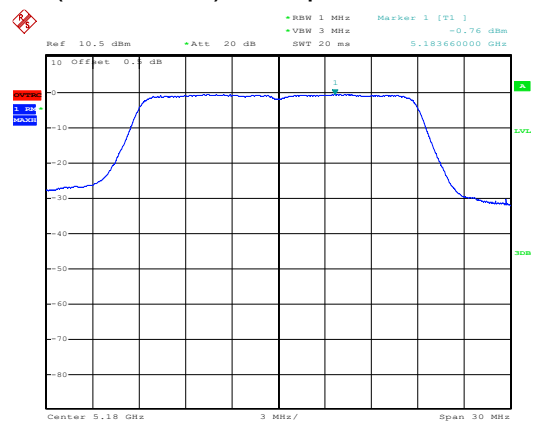
(802.11n20) PSD plot on channel 36
