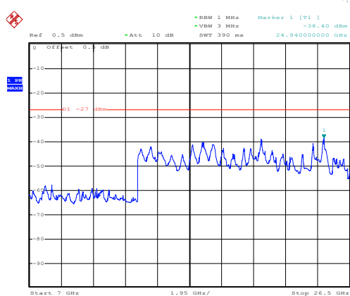
802.11ac20 on channel 165
