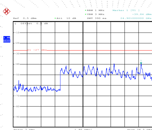
802.11a on channel 40
