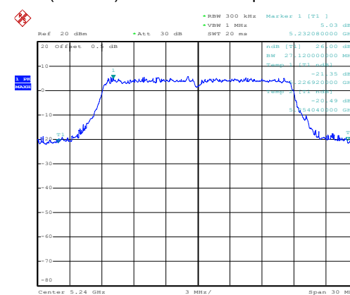
(802.11a) 26dB Bandwidth plot on channel 48
