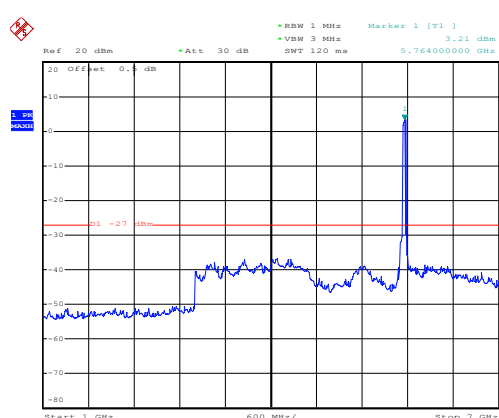
802.11ac40 on channel 151
