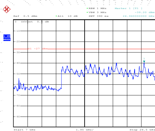
802.11n20 on channel 36
