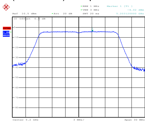
(802.11ac20) PSD plot on channel 40
