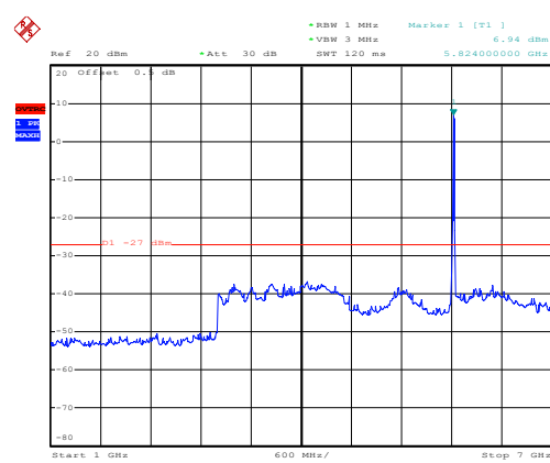
802.11n20 on channel 165
