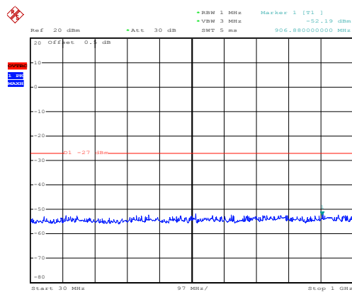
802.11n20 on channel 149
