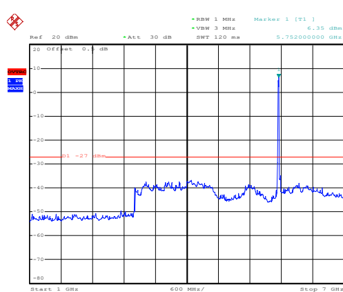
802.11n20 on channel 149
