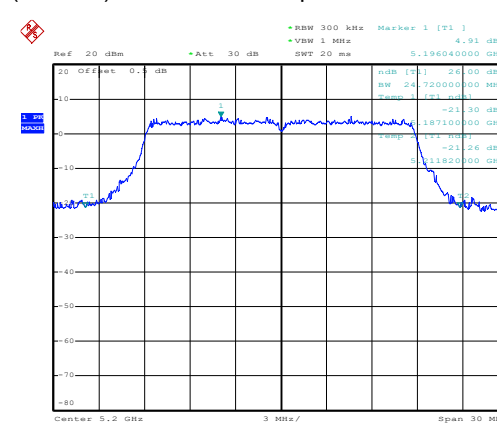
(802.11a) 26dB Bandwidth plot on channel 40
