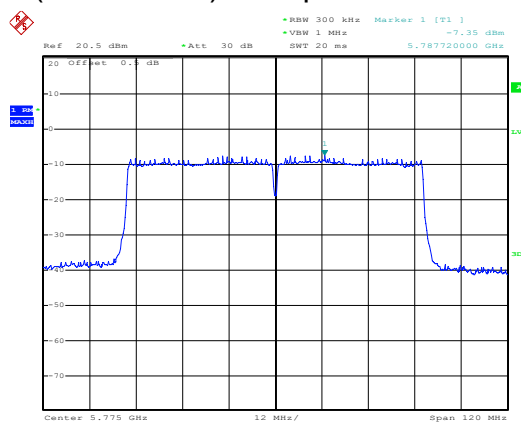
(802.11ac80) PSD plot on channel 155
