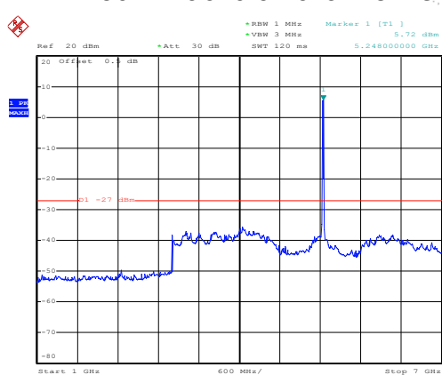
802.11ac20 on channel 48
