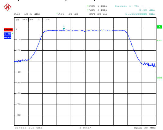
(802.11n20) PSD plot on channel 40
