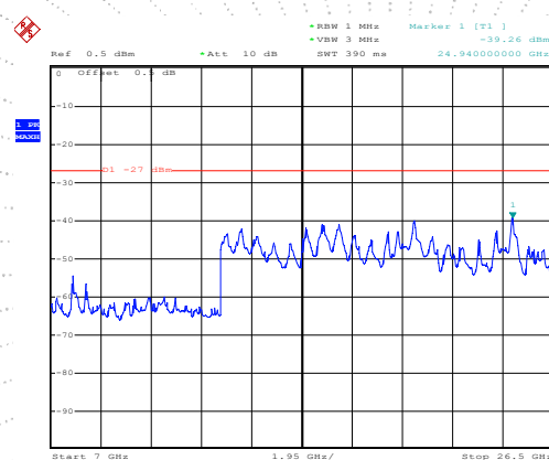
802.11n20 on channel 48
