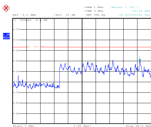
802.11n20 on channel 40
