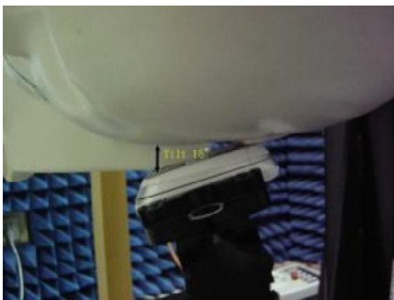
Fig.7 Photograph of the Left Hand Side Tilt ,off status
