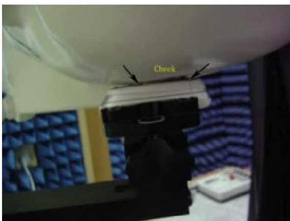
Fig.6 Photograph of the Left Hand Side Cheek,off status
