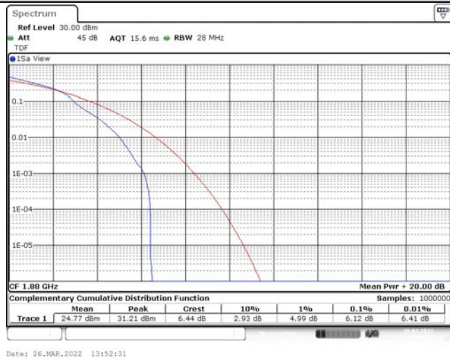
Band2-10MHz-16QAM-18900-1RB#0
