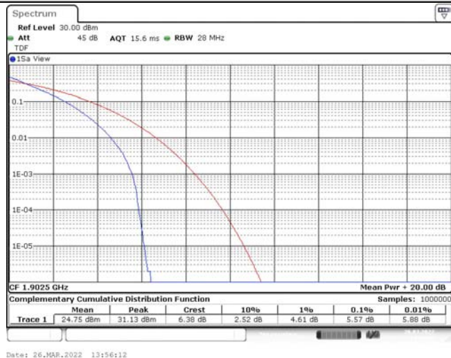
Band2-15MHz-QPSK-19125-75RB#0
