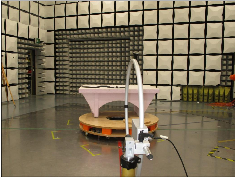
Test setup: Radiated measurements (9KHz -30MHz)
