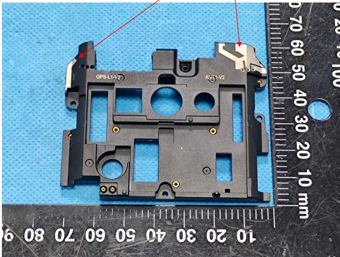
2.4G Wi-Fi/Bluetooth/GPS Antenna
