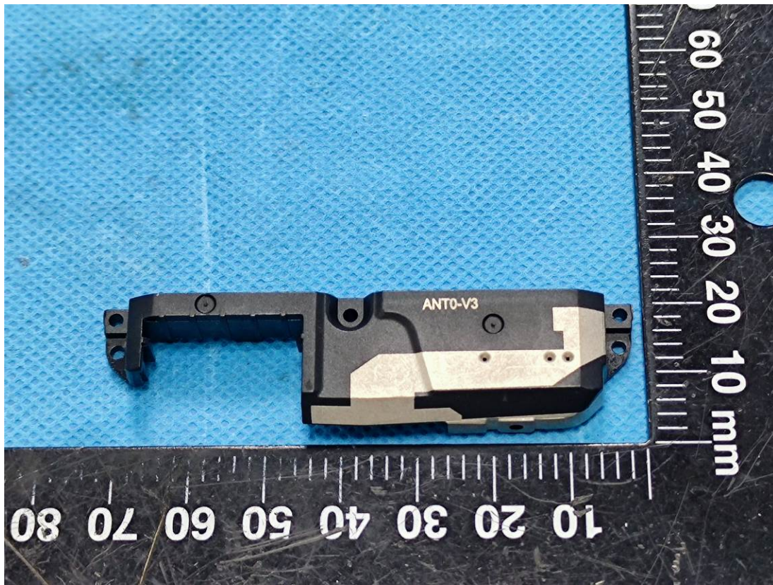
WWAN Main Antenna
