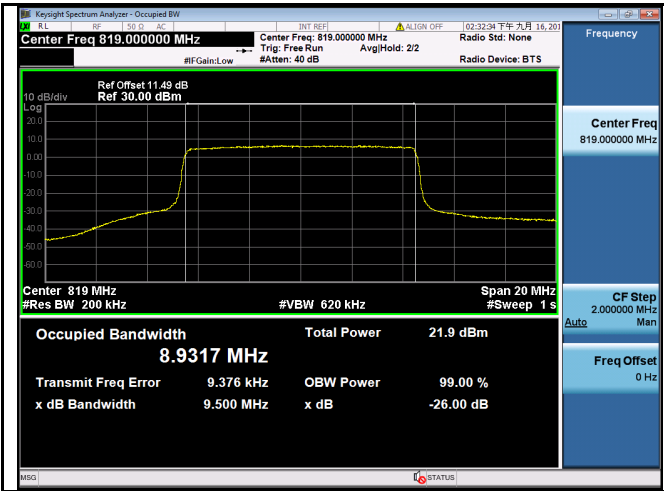
LTE band 26 - Low CH QPSK-10
