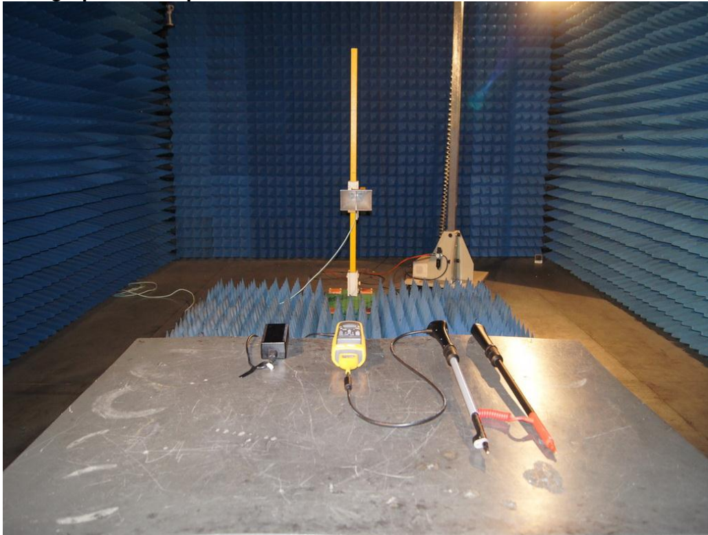
Photograph 3: Set-up for Radiated Emission – 1-18 GHz
