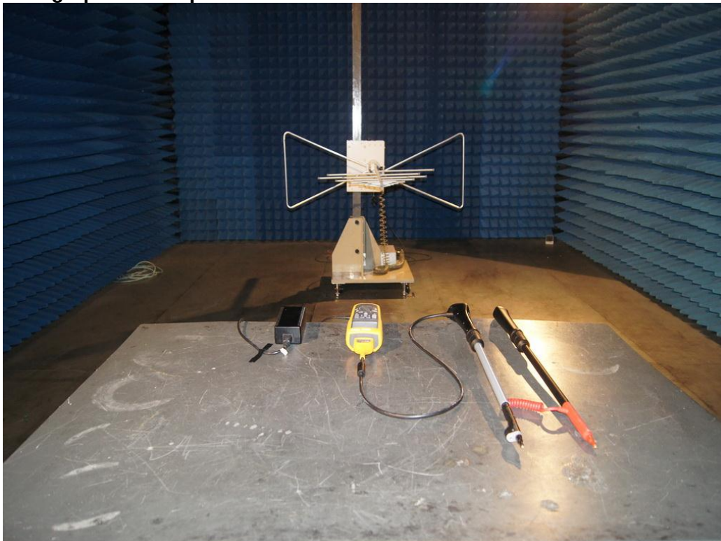
Photograph 2: Set-up for Radiated Emission – 30-1000 MHz
