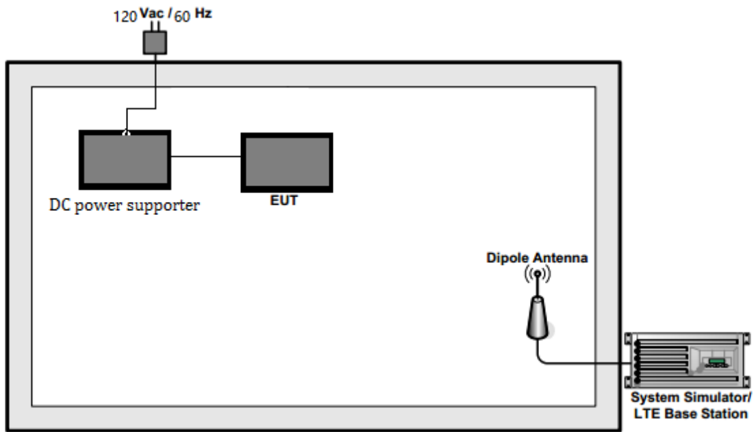
Radiated Setup
