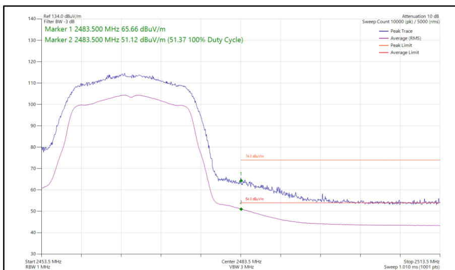
Figure 82 - 802.11n HT20, SISO, Core 1 - 2467 MHz Band Edge Frequency 2483.5 MHz
