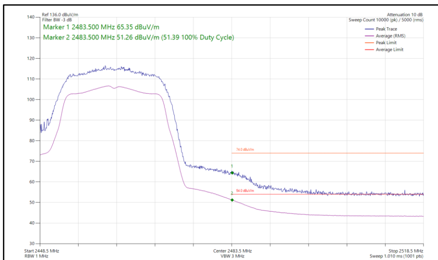
Figure 81 - 802.11n HT20, SISO, Core 1 - 2462 MHz Band Edge Frequency 2483.5 MHz
