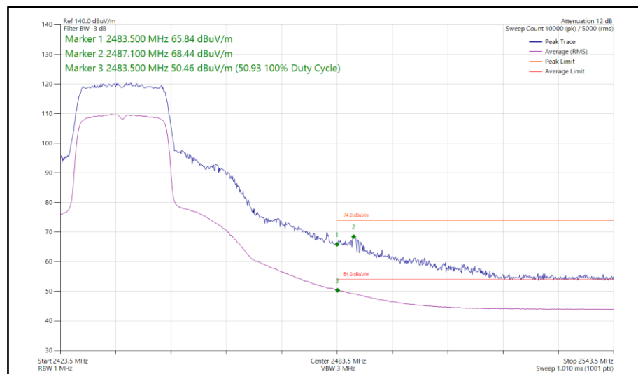
Figure 84 - 802.11ax HE20, SU, SISO, Core 1 - 2437 MHz Band Edge Frequency 2483.5 MHz
