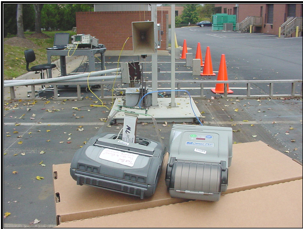
PHOTOGRAPH 7: RADIATED EMISSION REAR VIEW; WORST CASE CONFIGURATION CAMEO 3 PEP (CQ15729-1) ANTENNA
