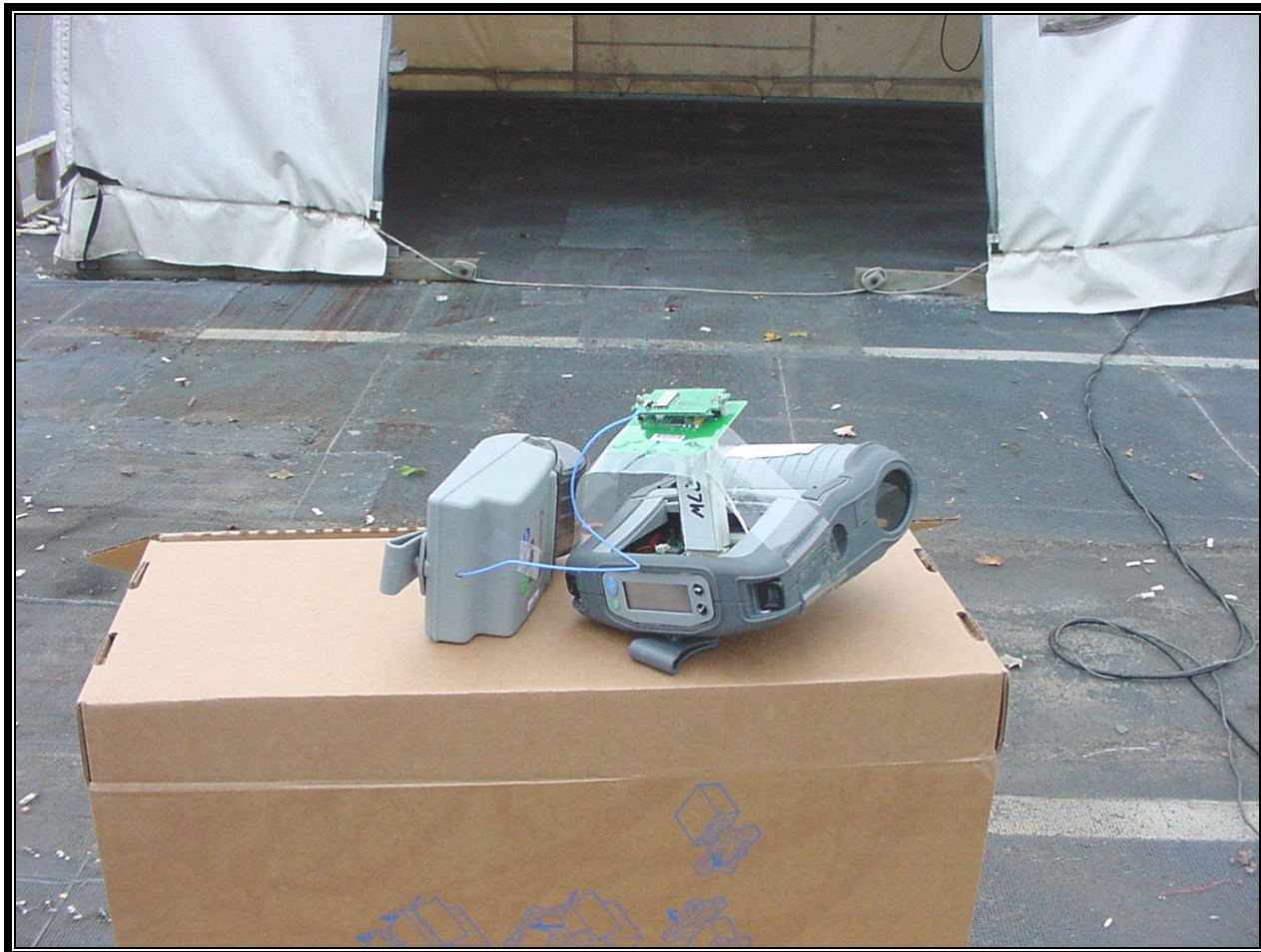
PHOTOGRAPH 8: RADIATED EMISSION FRONT VIEW, WORST CASE CONFIGURATION CAMEO 2 (CQ15731-1) ANTENNA
