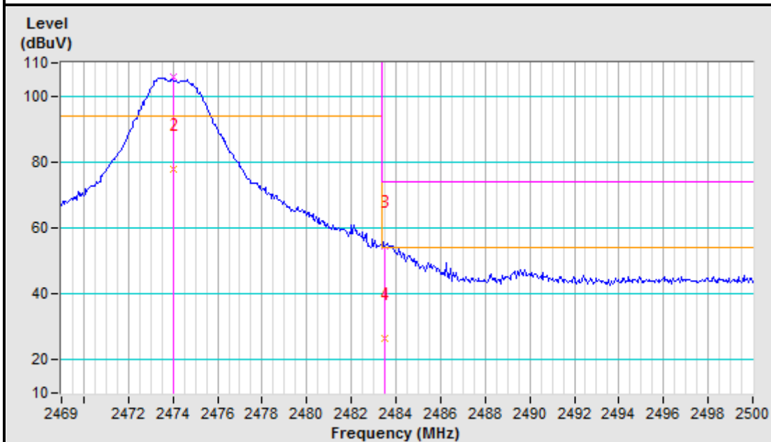
2474MHz Vertical
