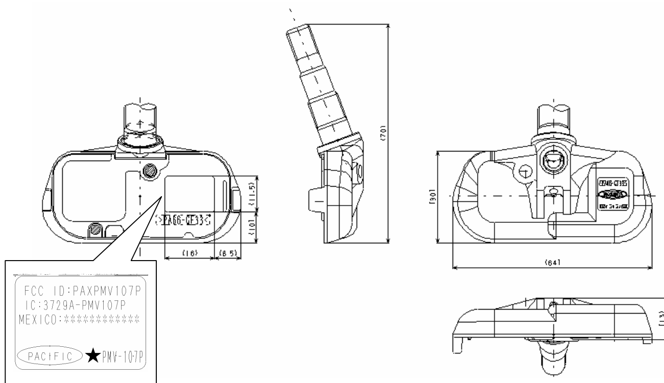
Fig 5. Marking location and dimension
