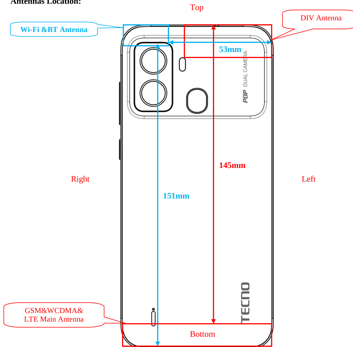
EUT Back View
