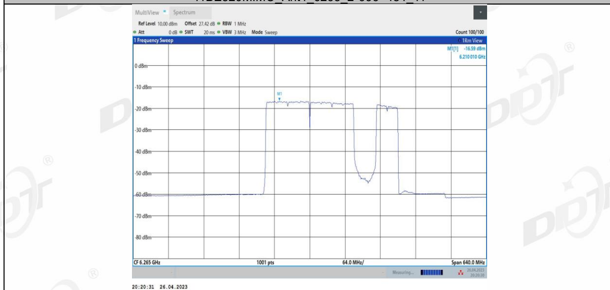
11BE320MIMO Ant4_6265_2*996+484_12
