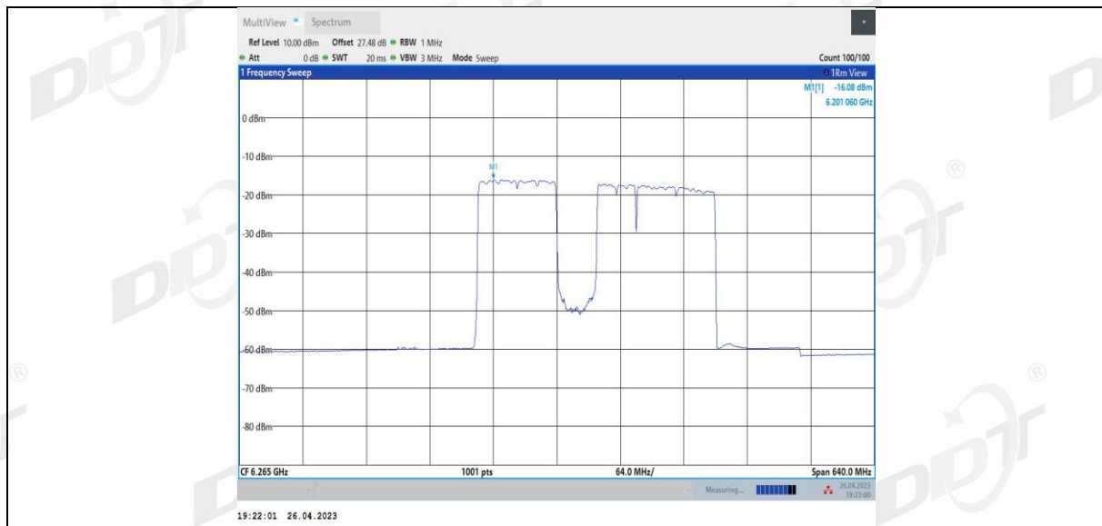
11BE320MIMO Ant1_6265_2*996+484_10
