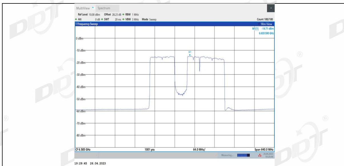
11BE320MIMO Ant3_6585_2*996+484_10
