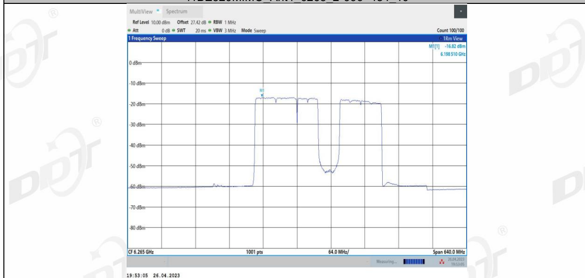
11BE320MIMO Ant4_6265_2*996+484_11
