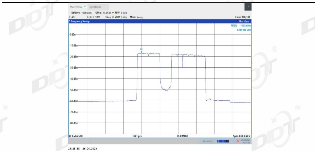
11BE320MIMO Ant4_6265_2*996+484_10
