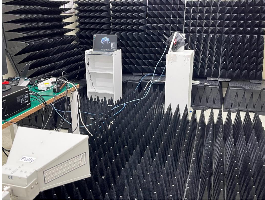
Photograph 18: Test Setup for DFS (Back View)
