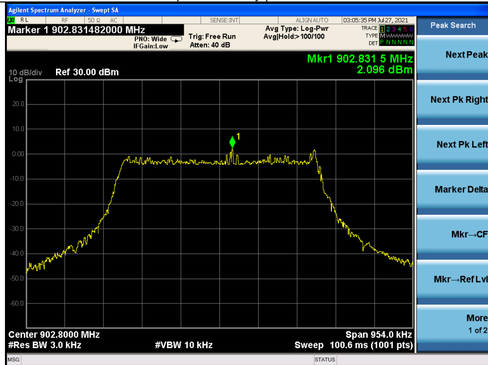
Power spectral density plot on 902.8MHz
