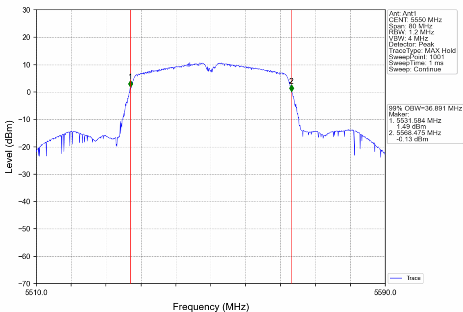
802.11n(HT40)_MCH_5550MHz_Ant1_NTNV
