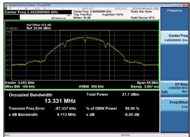
6dB Bandwidth-802.11b,2462MHz,Ant1
