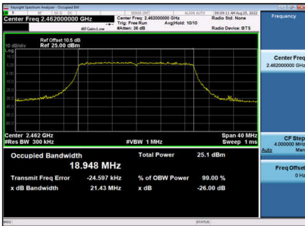
99% Bandwidth-802.11ax(HE20),2462MHz ,Ant0
