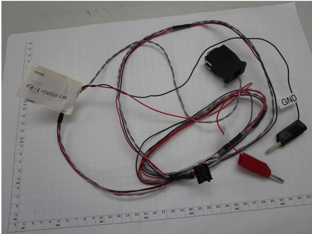
Photograph 9 Auxillary harness
