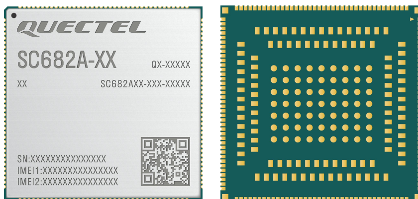
Figure 44: Top and Bottom Views of SC682A Series
