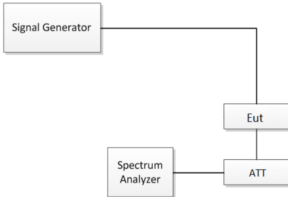
Fig.6. Spurious emissions at RF antenna connector
