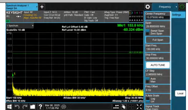
Band13-10MHz-QPSK-23230-1RB#0-0.15~30-PASS
