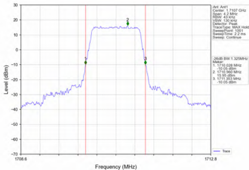
Band4_1.4MHz_256QAM_LCH_1710.7MHz_RB_6_0_NTNV
