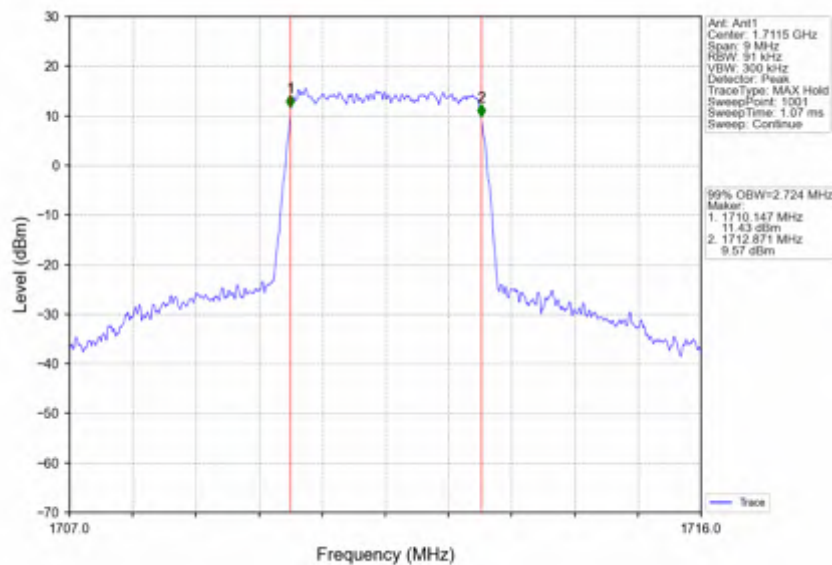
Band4_3MHz_256QAM_LCH_1711.5MHz_RB_15_0_NTNV
