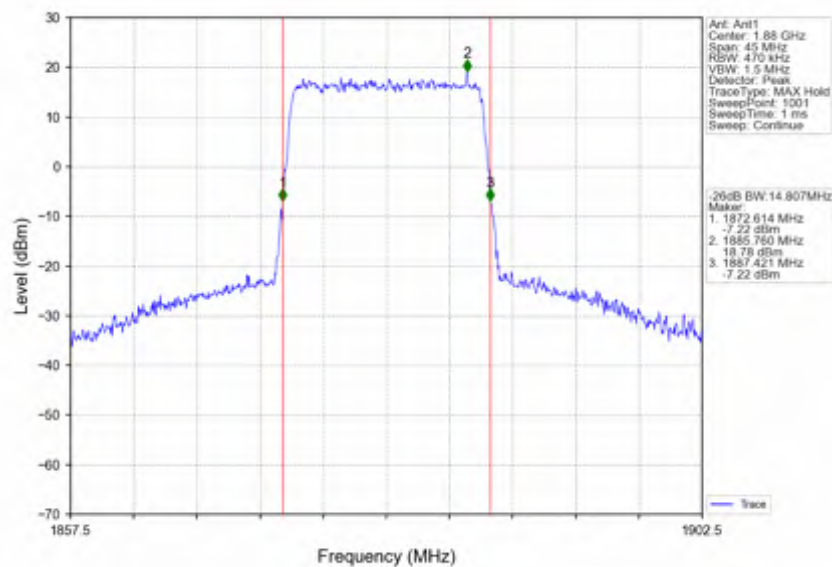
Band2_15MHz_64QAM_MCH_1880MHz_RB_75_0_NTNV
