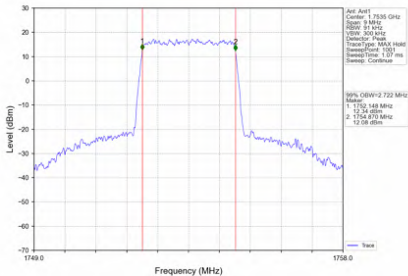
Band4_3MHz_16QAM_HCH_1753.5MHz_RB_15_0_NTNV
