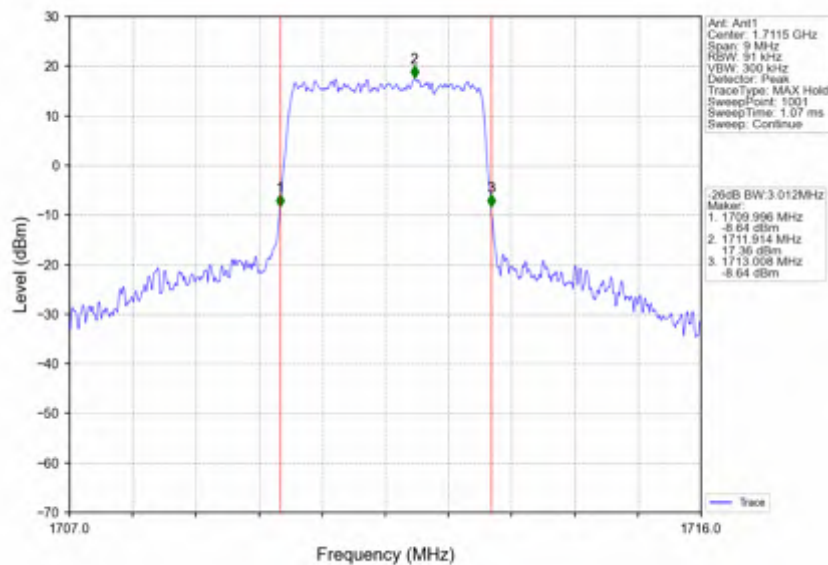
Band4_3MHz_16QAM_LCH_1711.5MHz_RB_15_0_NTNV
