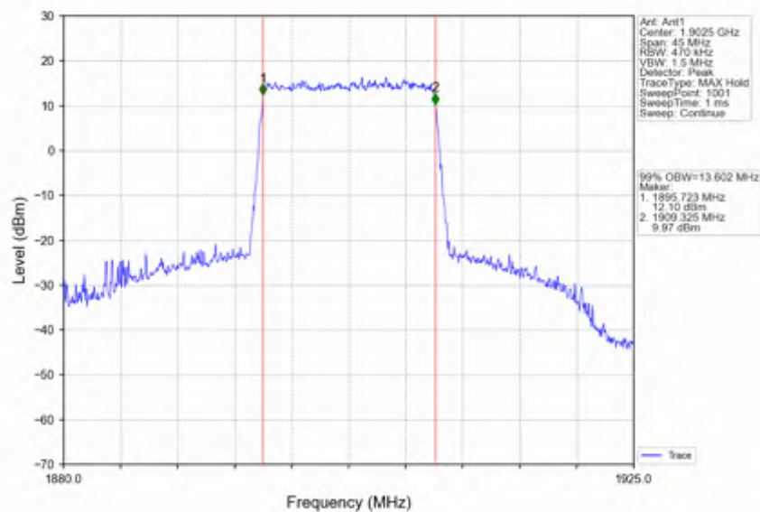
Band2_15MHz_256QAM_HCH_1902.5MHz_RB_75_0_NTNV
