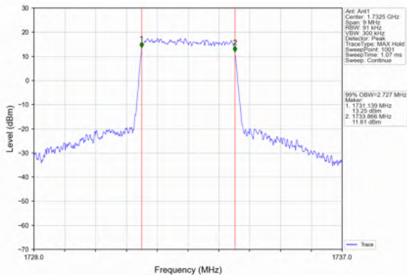
Band4_3MHz_64QAM_MCH_1732.5MHz_RB_15_0_NTNV
