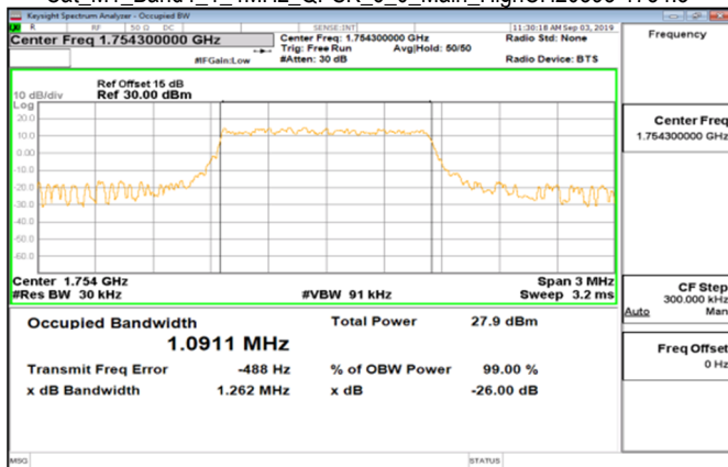
Cat M1_Band4_1_4MHz_QPSK_6_0_Main_HighCH20393-1754.3
