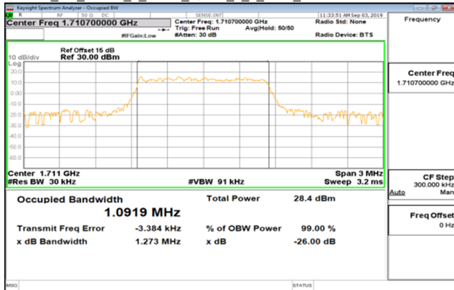
Cat M1_Band4_1_4MHz_QPSK_6_0_Main_LowCH19957-1710.7
