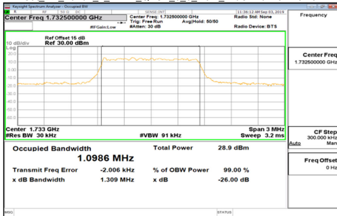
Cat M1_Band4_1_4MHz_QPSK_6_0_Main_MidCH20175-1732.5
