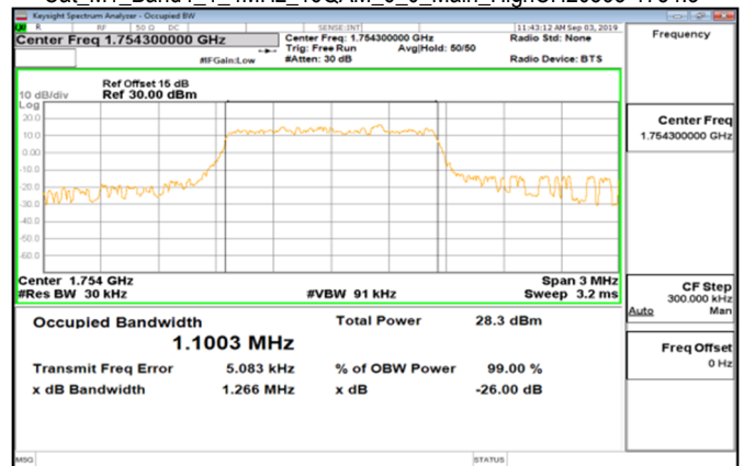
Cat M1_Band4_1_4MHz_16QAM_6_0_Main_HighCH20393-1754.3
