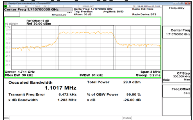
Cat M1_Band4_1_4MHz_16QAM_6_0_Main_LowCH19957-1710.7
