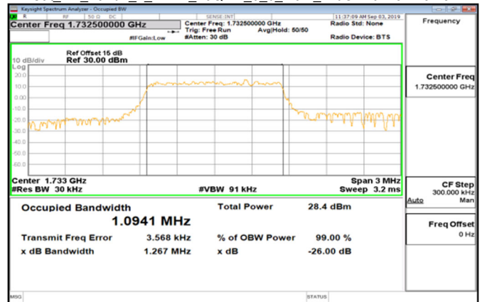
Cat M1_Band4_1_4MHz_16QAM_6_0_Main_MidCH20175-1732.5
