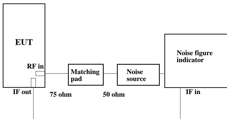
Figure 6. Noise figure
