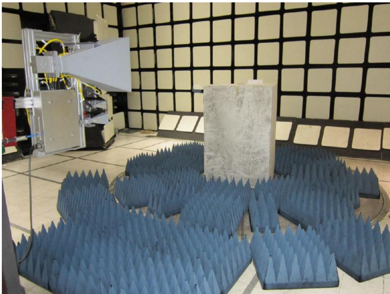
Radiated Testing Above 1GHz - Front View
