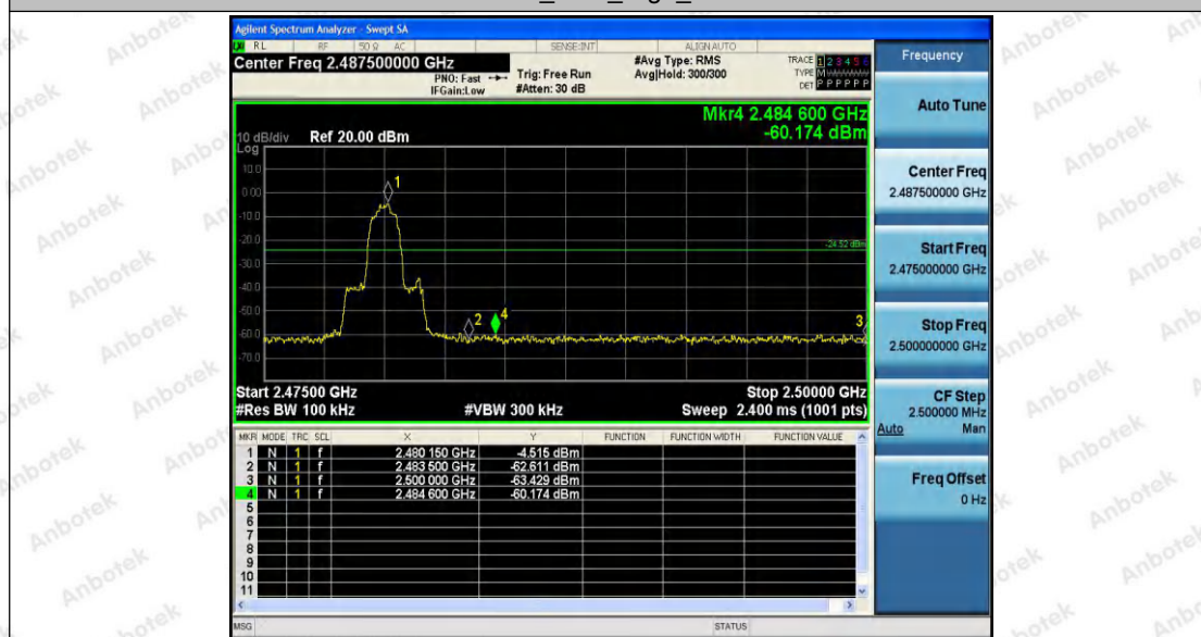
3DH5_Ant1_High_2480
