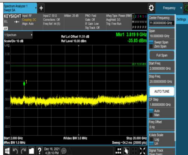
Band2-1.4MHz-16QAM-19193-6RB#0-Range3:2000~20000MHz
