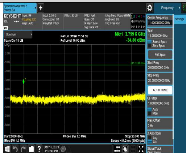
Band2-3MHz-QPSK-18900-15RB#0-Range3:2000~20000MHz
