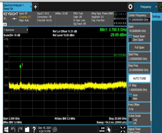
Band2-1.4MHz-QPSK-18900-6RB#0-Range3:2000~20000MHz
