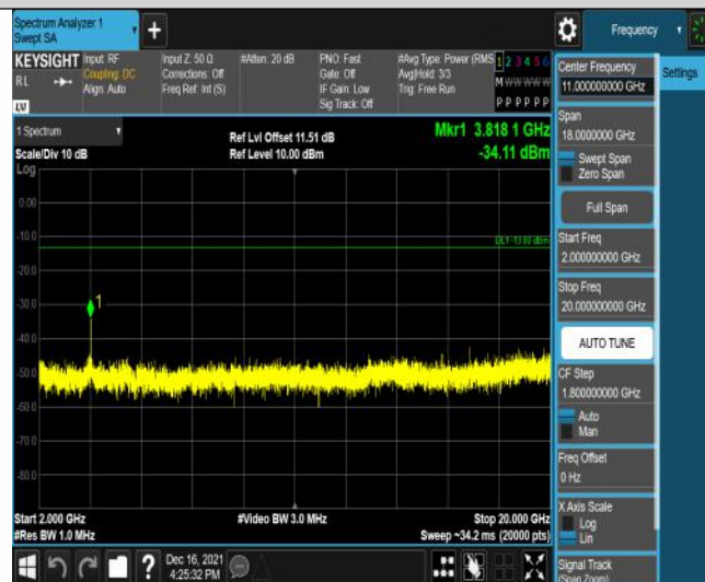
Band2-1.4MHz-QPSK-19193-6RB#0-Range3:2000~20000MHz
