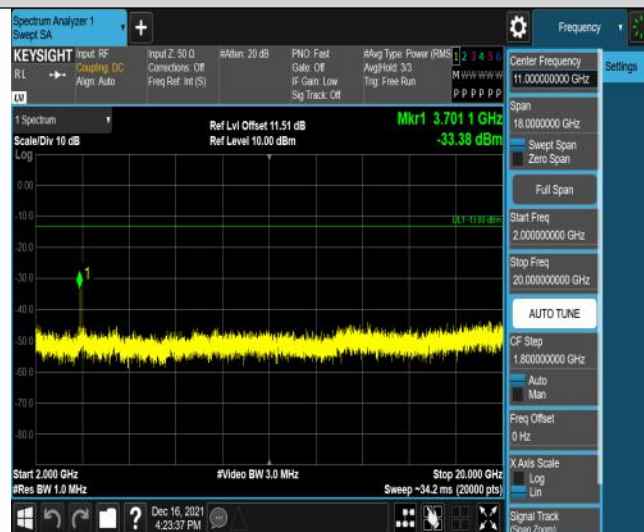
Band2-1.4MHz-16QAM-18607-6RB#0-Range3:2000~20000MHz
