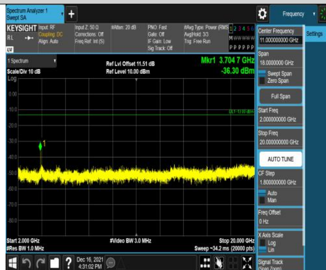
Band2-3MHz-16QAM-18615-15RB#0-Range3:2000~20000MHz
