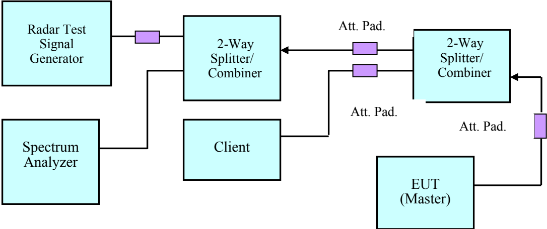
Conducted Calibration Setup Block Diagram
