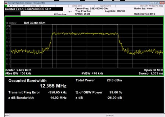
N41(15M)_DFT-s-OFDM_PI_2- BPSK Outer Full High CH
