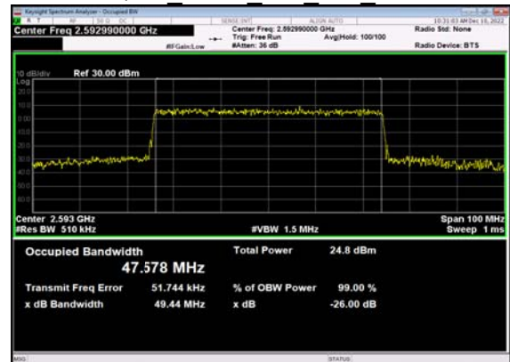
N41(50M)_CP-OFDM_64 QAM Outer Full Mid CH
